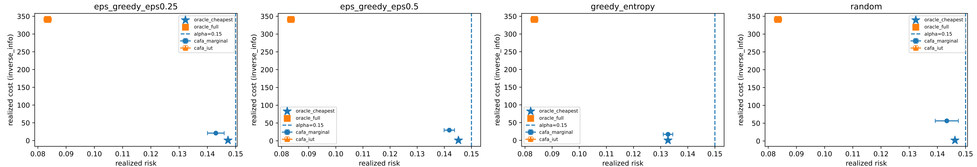
F1 realized (risk, cost) -- tabular-MiniBooNE ts0 (lambda_ref=0.9)
