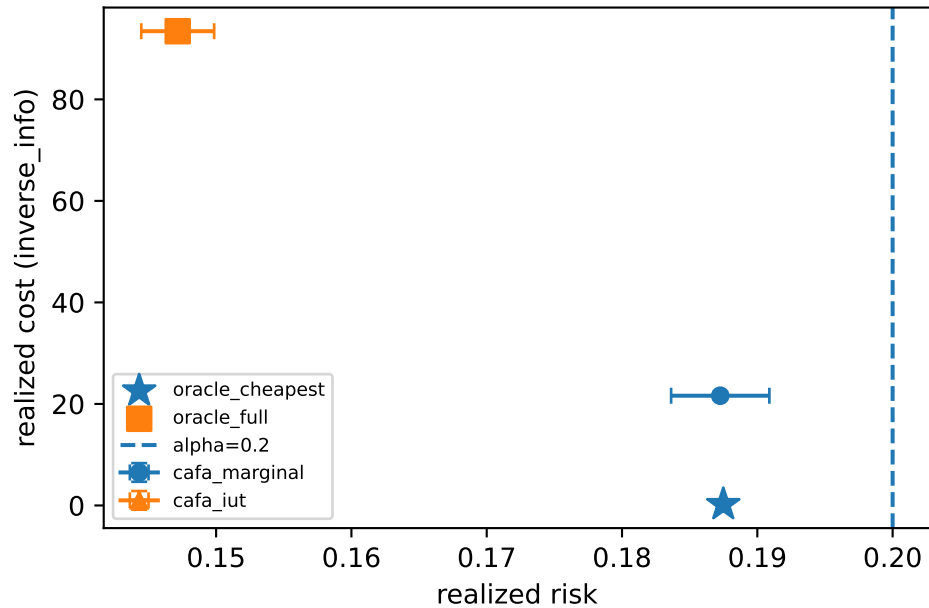
random
