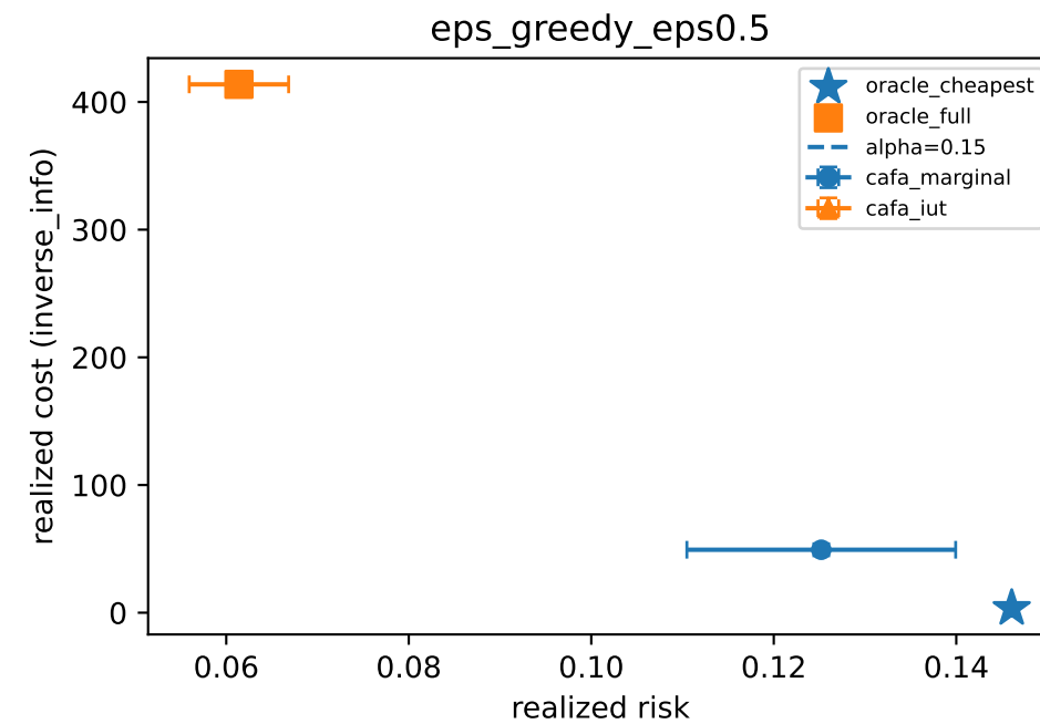
F1 realized (risk, cost) -- tabular-spambase ts0 (lambda_ref=0.9)
