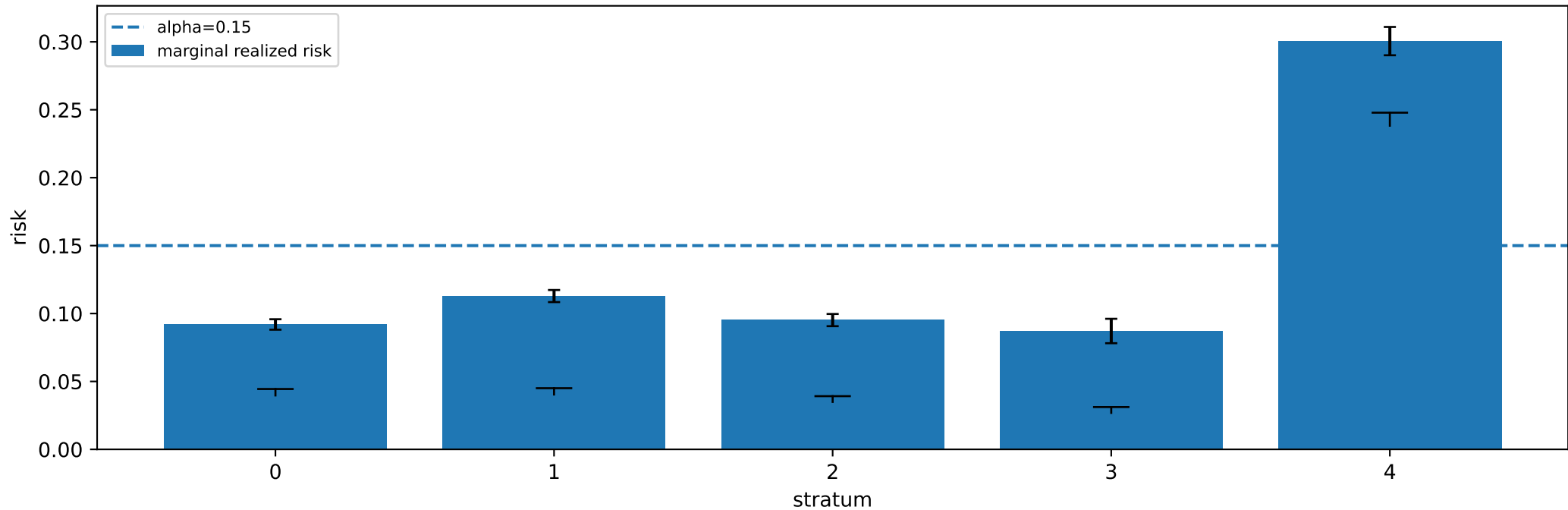
F2 per-stratum marginal risk -- mnist ts0 greedy lambda_ref=0.9
