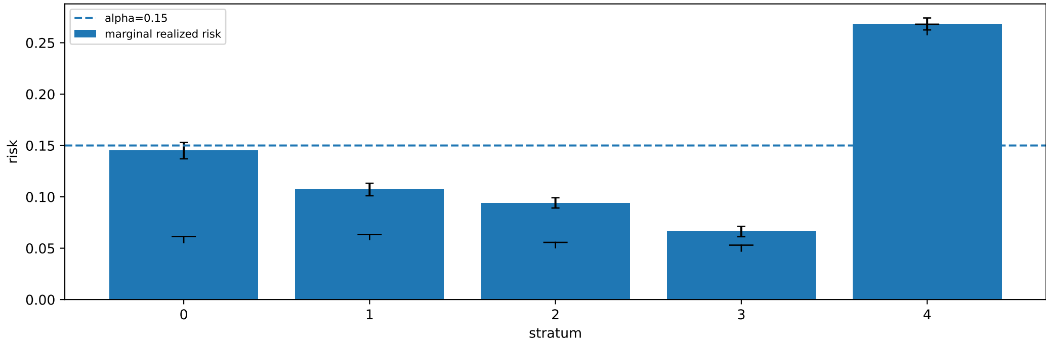
F2 per-stratum marginal risk -- mnist ts2 greedy lambda_ref=0.9
