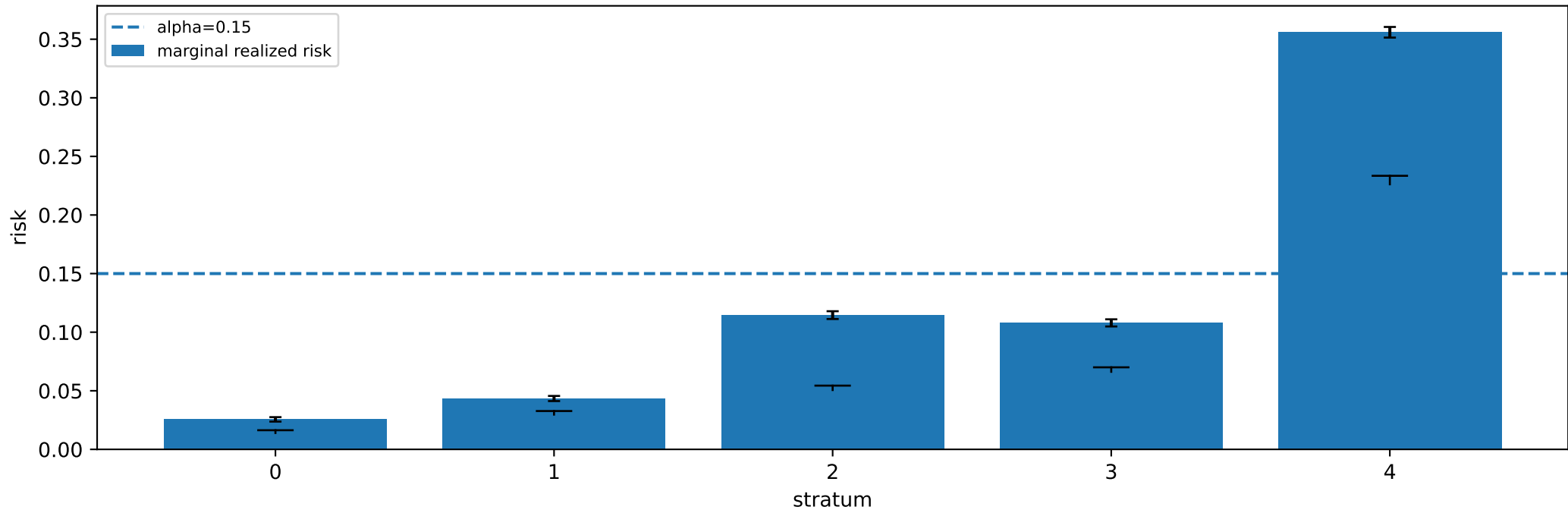
F2 per-stratum marginal risk -- tabular-MiniBooNE ts0 greedy lambda_ref=0.9
