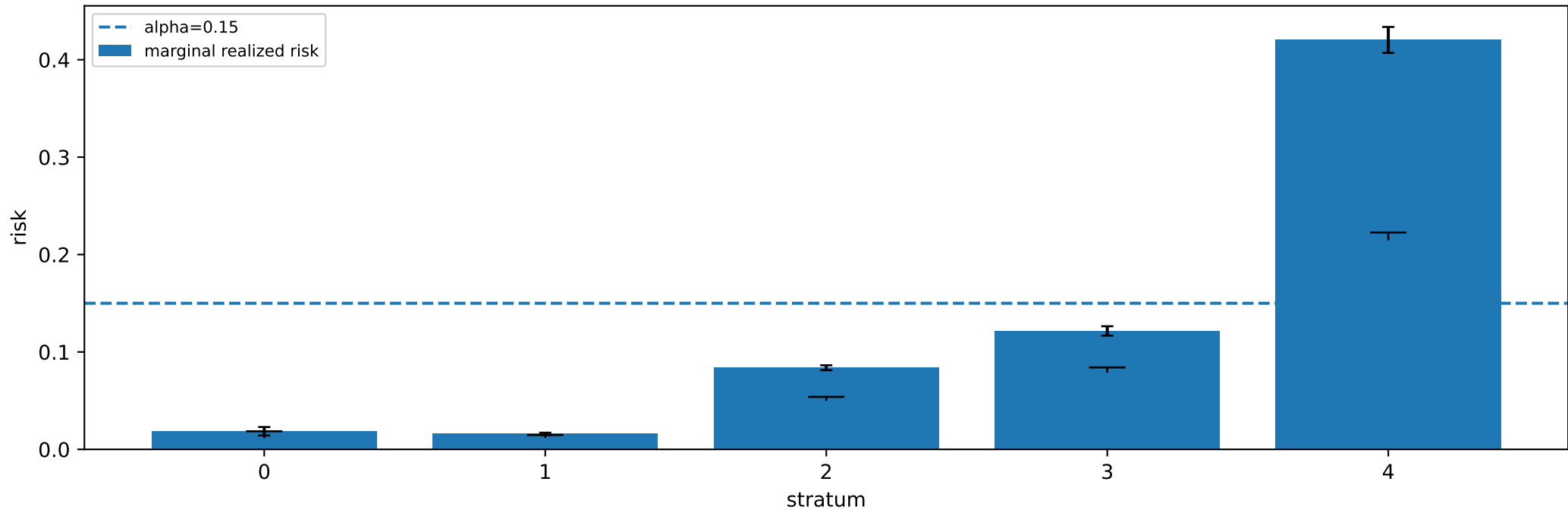
F2 per-stratum marginal risk -- tabular-MiniBooNE ts1 greedy lambda_ref=0.9
