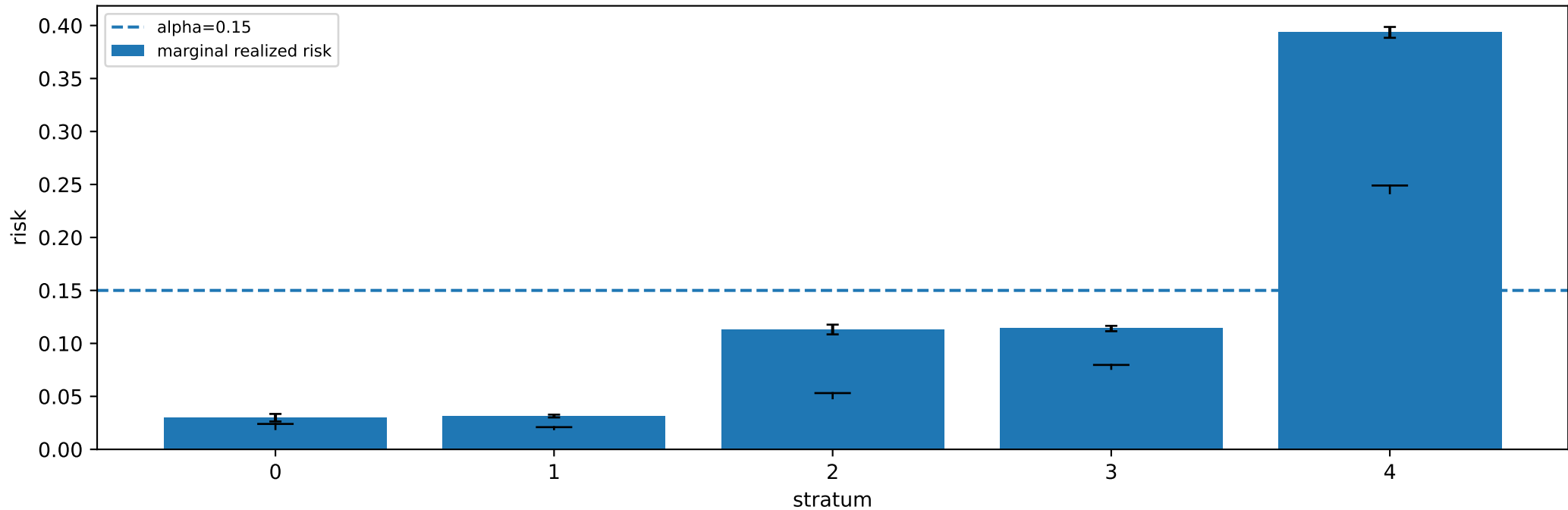
F2 per-stratum marginal risk -- tabular-MiniBooNE ts2 greedy lambda_ref=0.9
