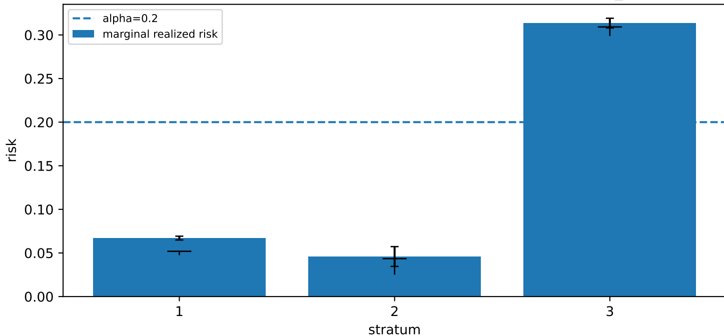
F2 per-stratum marginal risk -- tabular-adult ts0 greedy lambda_ref=0.9
