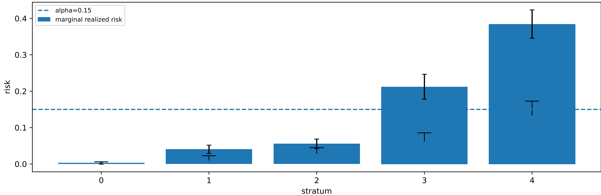
F2 per-stratum marginal risk -- tabular-spambase ts0 greedy lambda_ref=0.9
