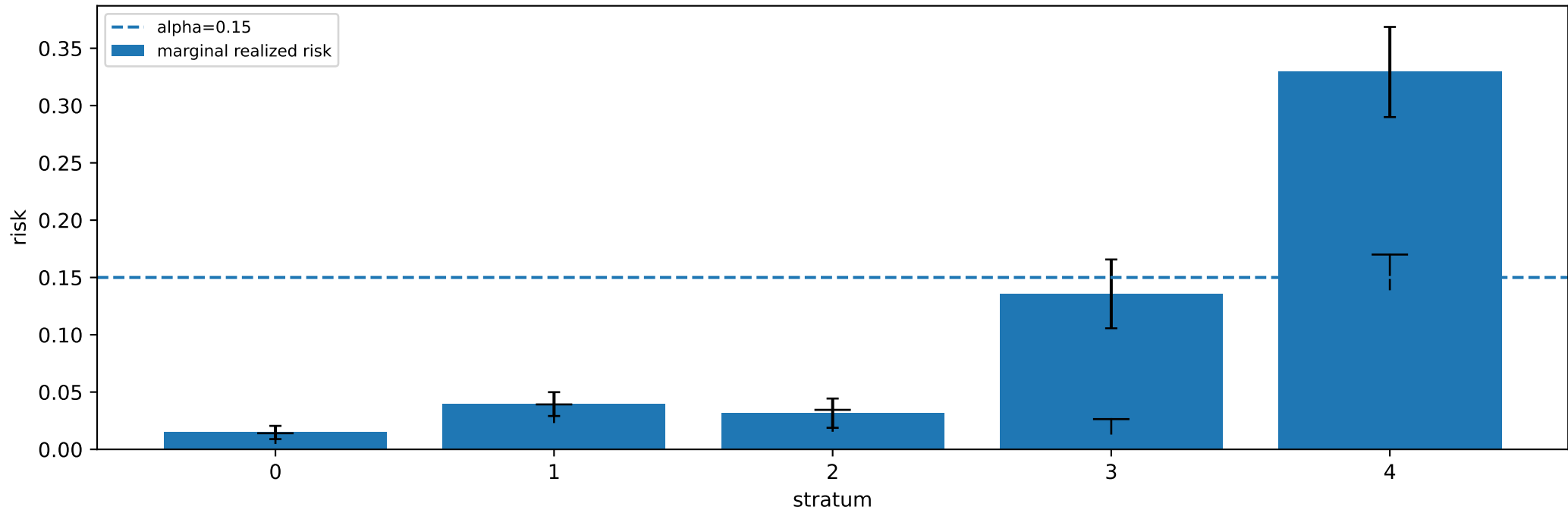
F2 per-stratum marginal risk -- tabular-spambase ts1 greedy lambda_ref=0.9
