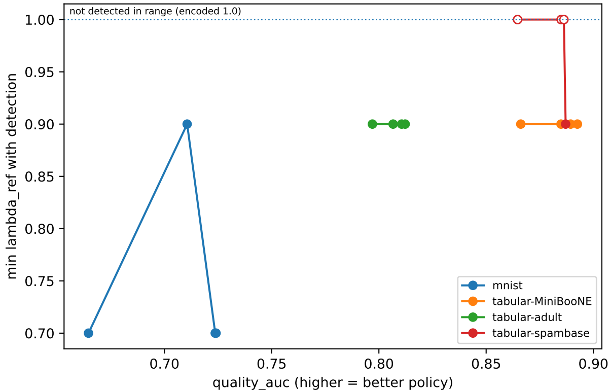
F3 (phase 2) detection frontier vs policy quality (ts0)
