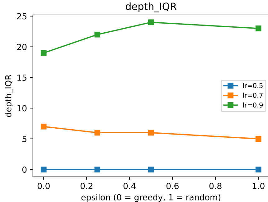
F3 (phase 2) concentration vs epsilon -- tabular-spambase ts0
