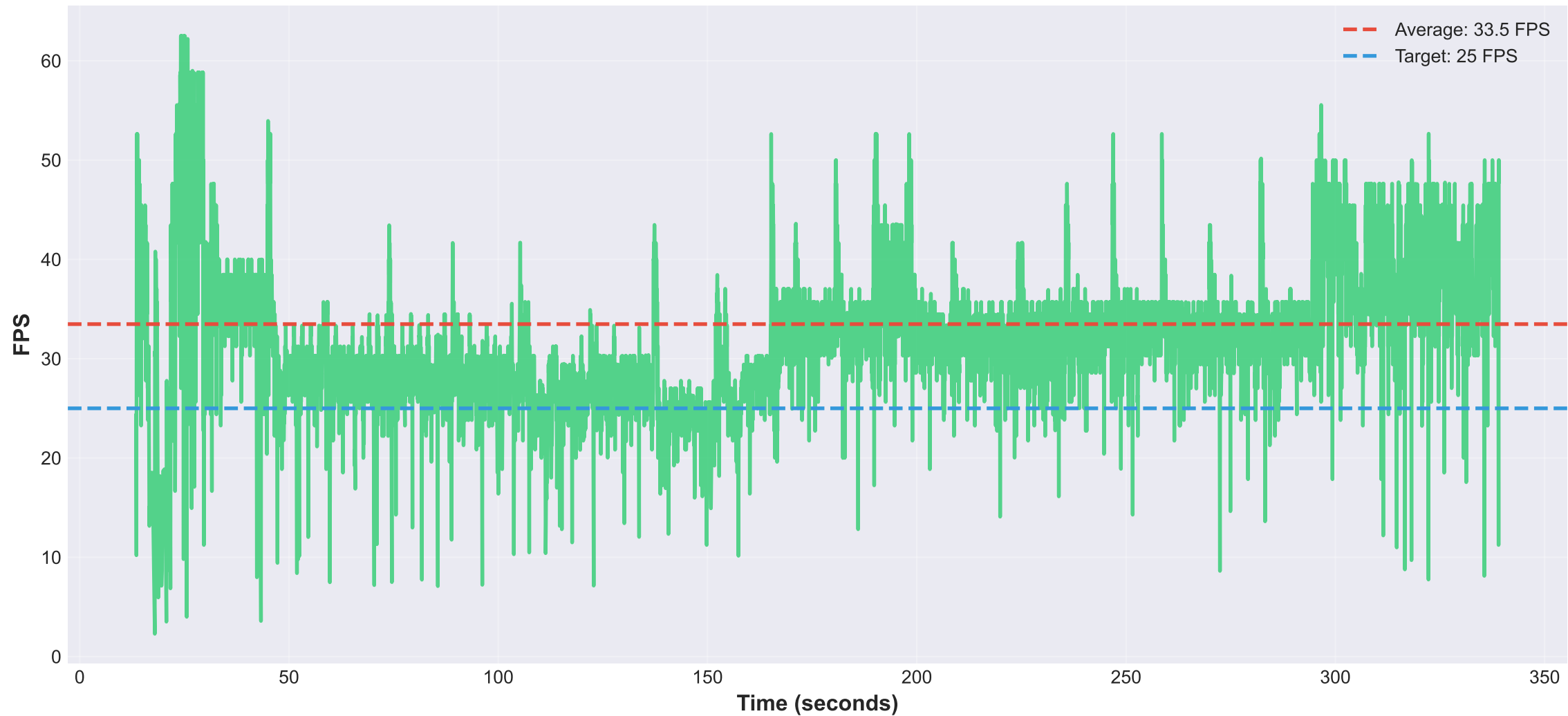
Real-Time Pipeline Performance (FPS Over Time)
