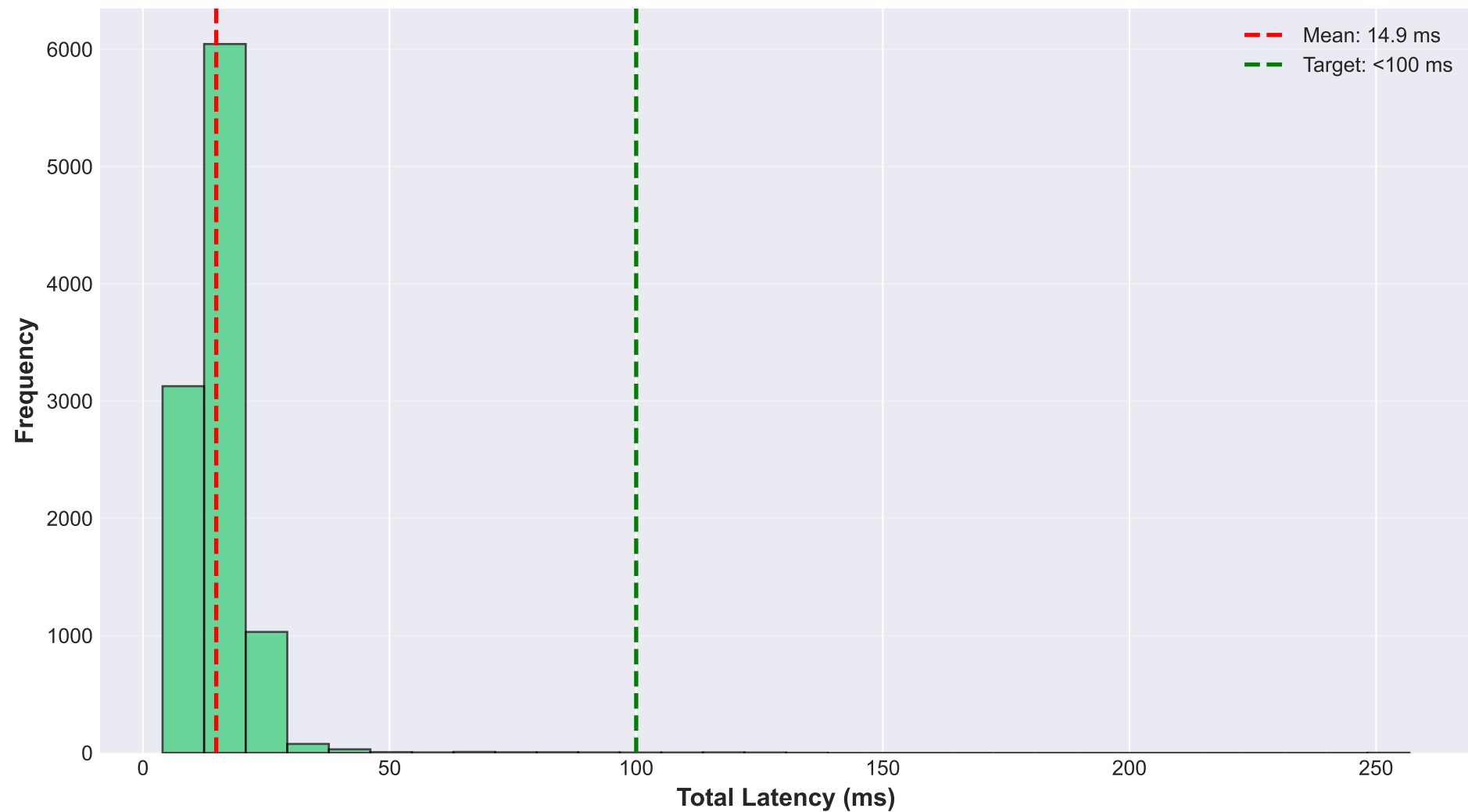
Per-Frame Latency Distribution
