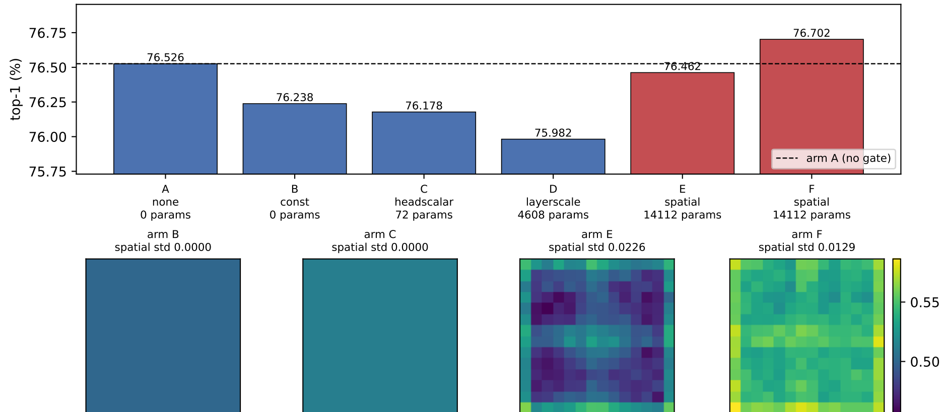
(a) ViT-S/16, mixup, seed 0, 100 EPOCHS — one seed per arm; the 300-epoch headline is a different schedule source: exact fp32, full 50k val (tools/eval.py)
