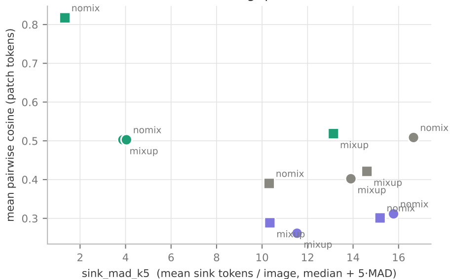
Oversmoothing (pairwise)
