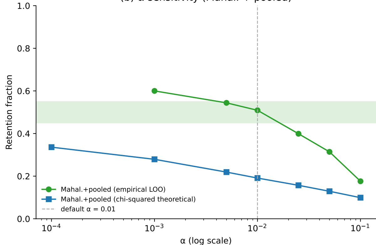
(b) \alpha -sensitivity (Mahal. + pooled)
