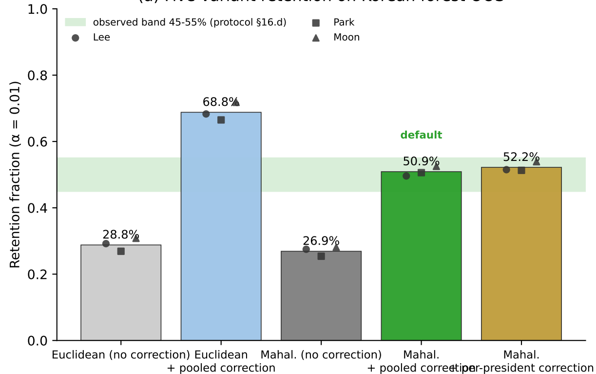
(a) Five-variant retention on Korean forest OOS
