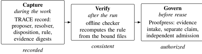
Fig. 1. One decision across the three boundaries. The arrows carry the record and the check result, never a status: recorded is not verified, consistent is not authentic, and neither is authorized for reuse.
