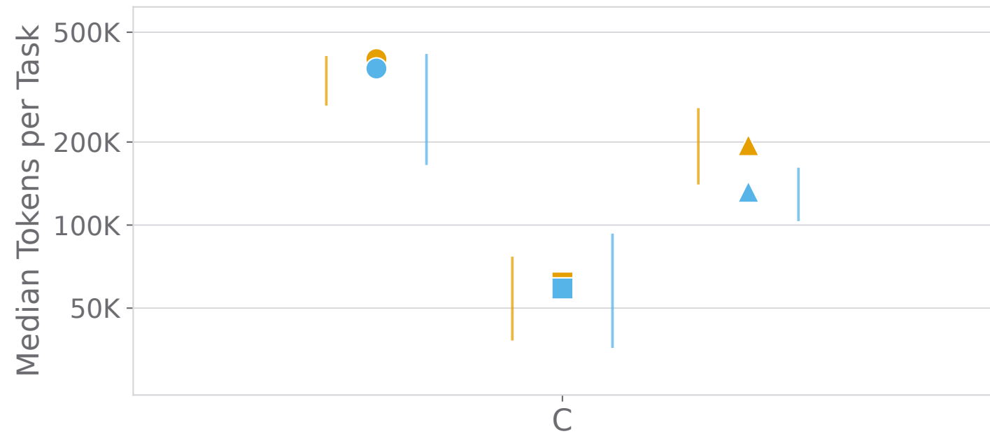
Repository vs Kernel, Scientific Computing
