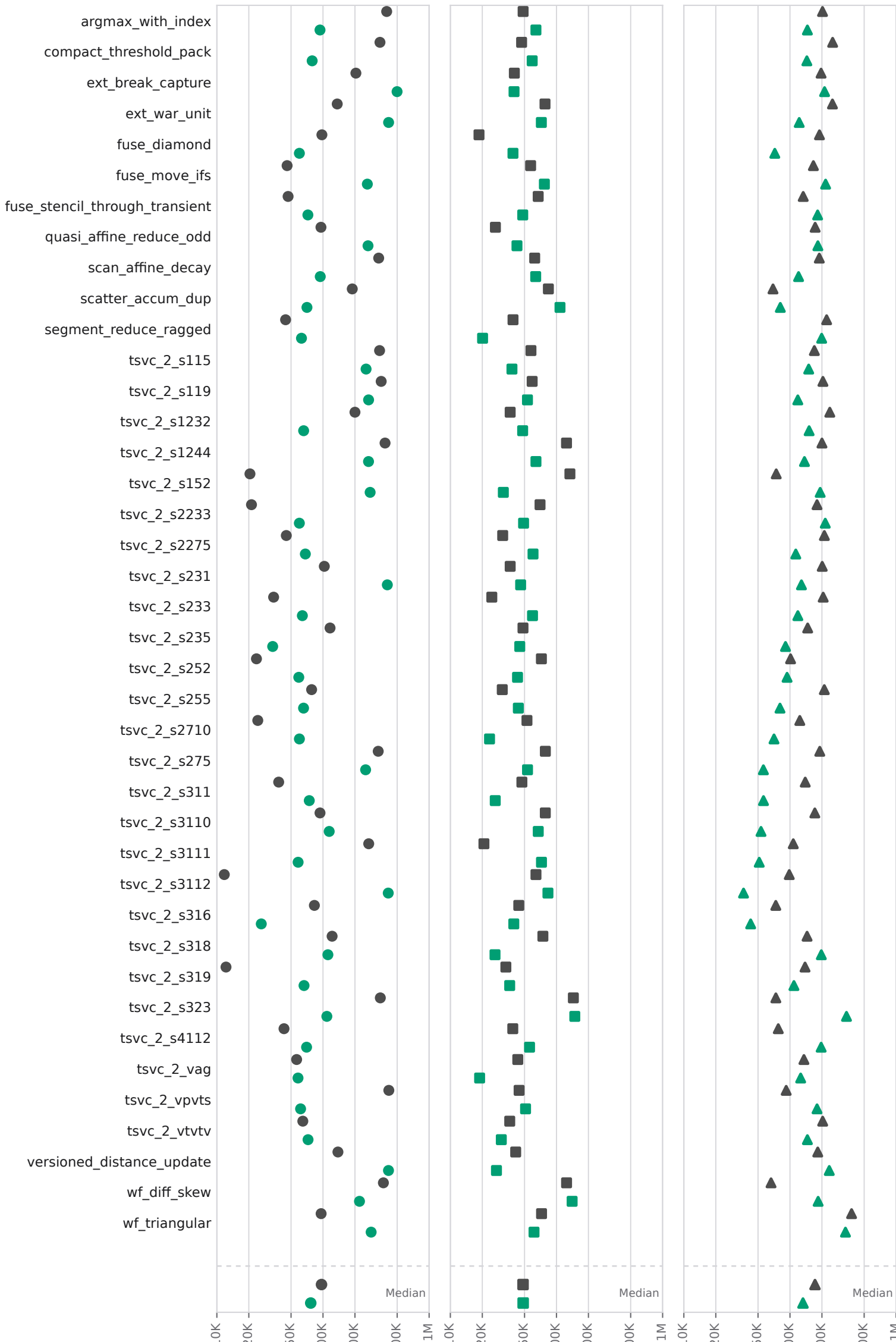
Tokens Spent
