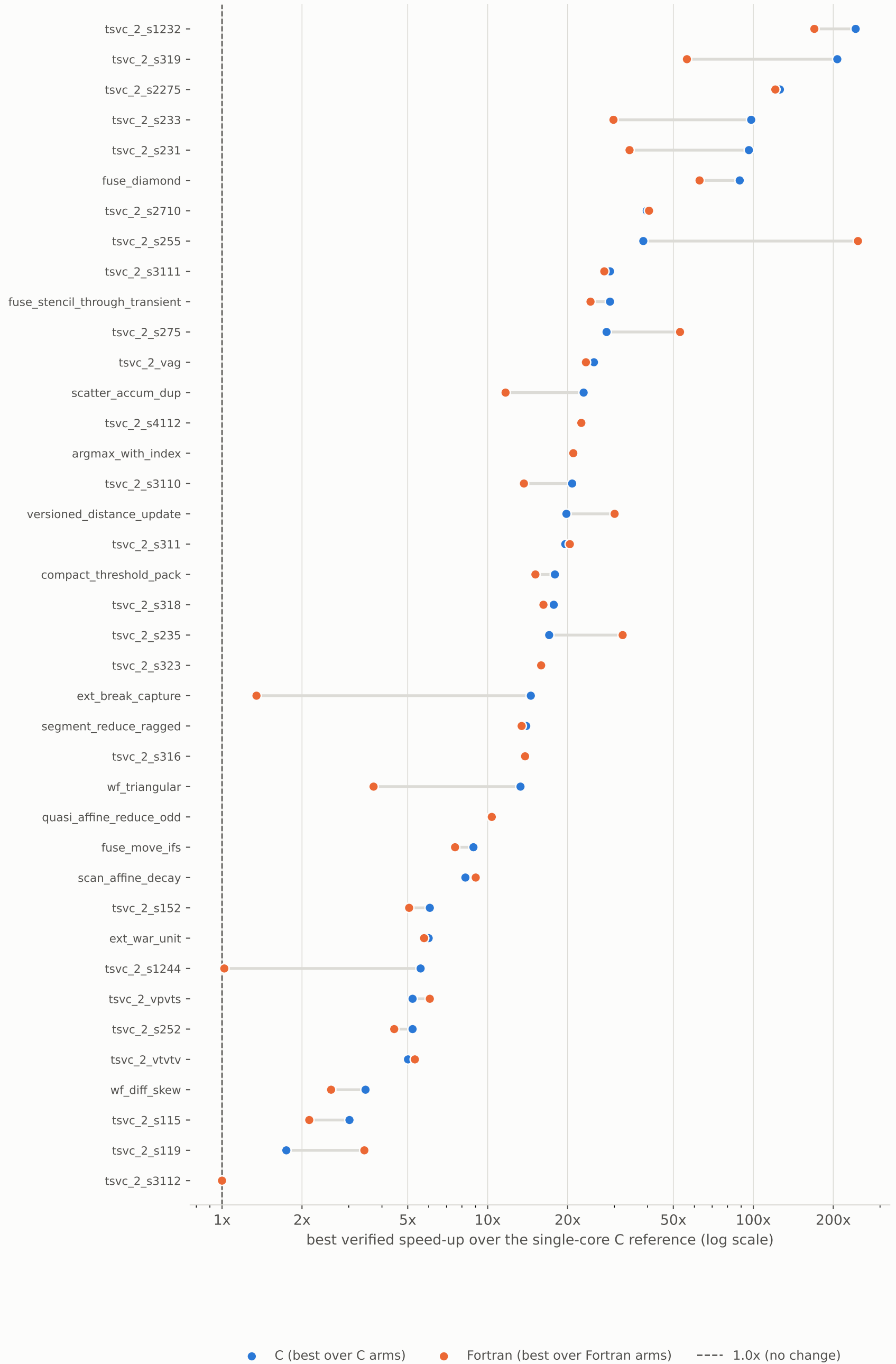
llr40: best agent speed-up per kernel, C against Fortran
