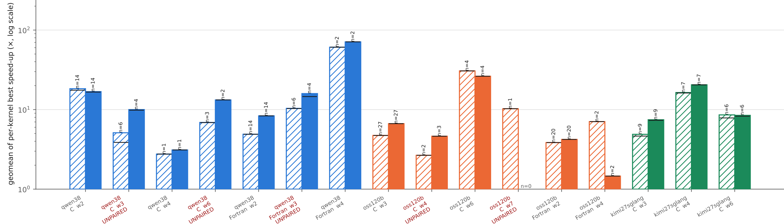
Speed-up with and without the skills packet, aggregated per kernel
