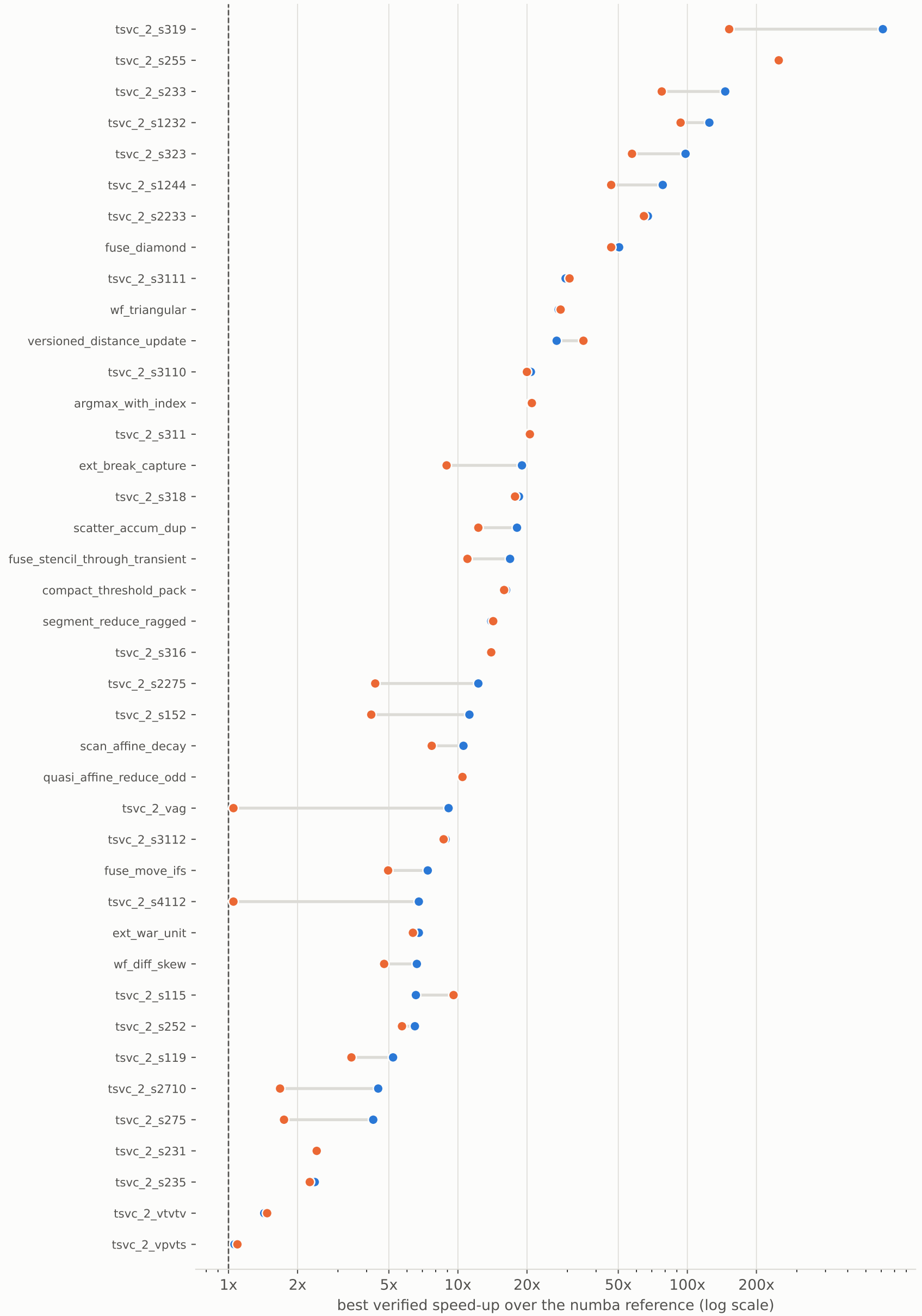
llr40: best agent speed-up per kernel, C against Fortran (vs numba)
