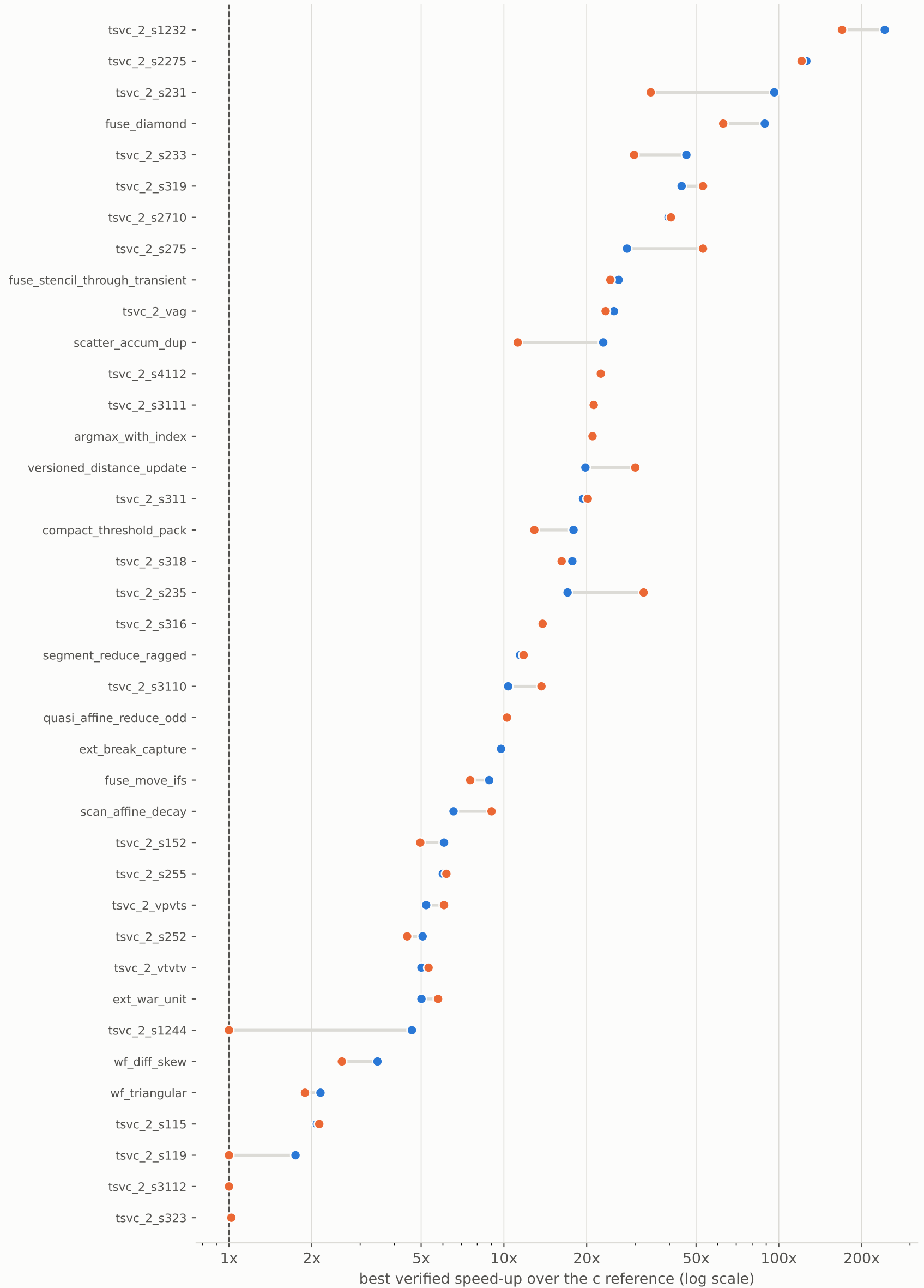
llr40: best agent speed-up per kernel, C against Fortran (vs c)
