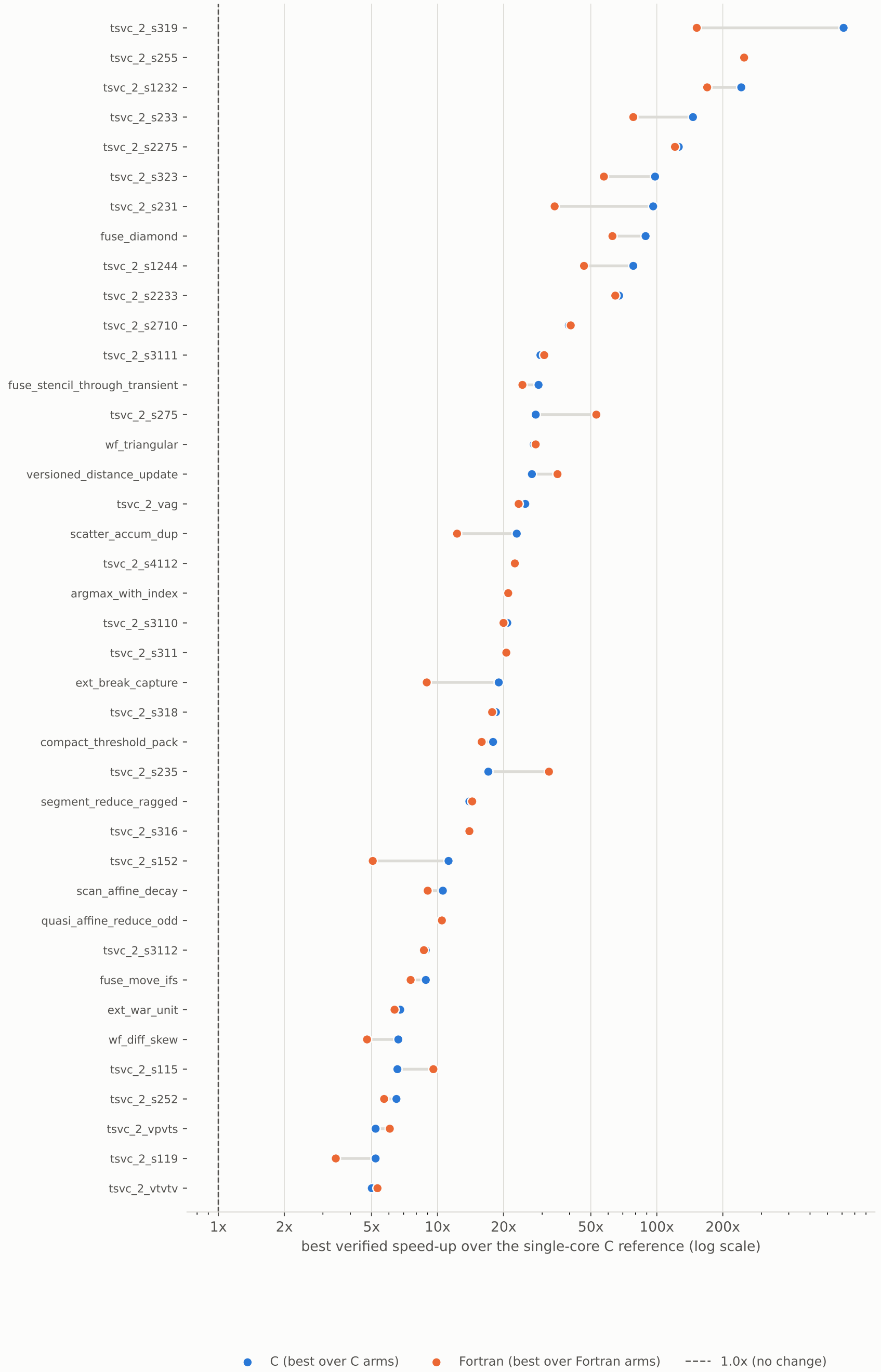
llr40: best agent speed-up per kernel, C against Fortran
