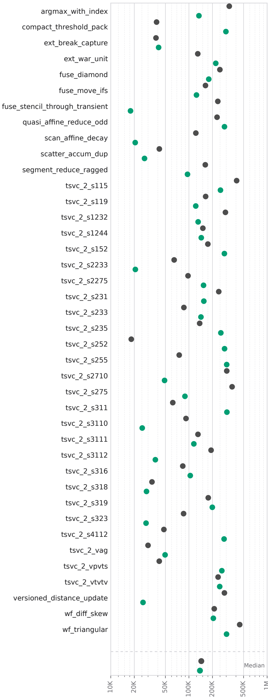
Tokens Spent
