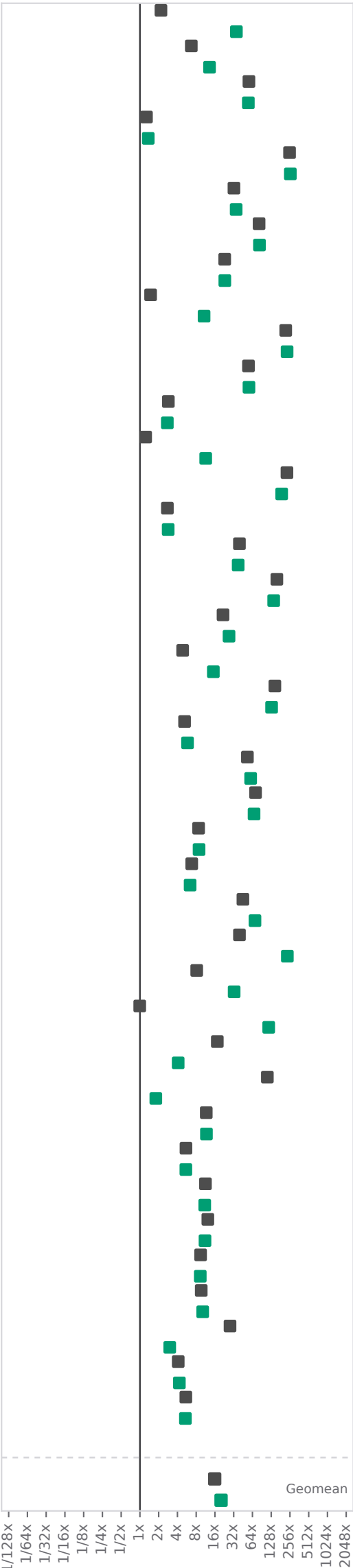
GPT-OSS-120B
