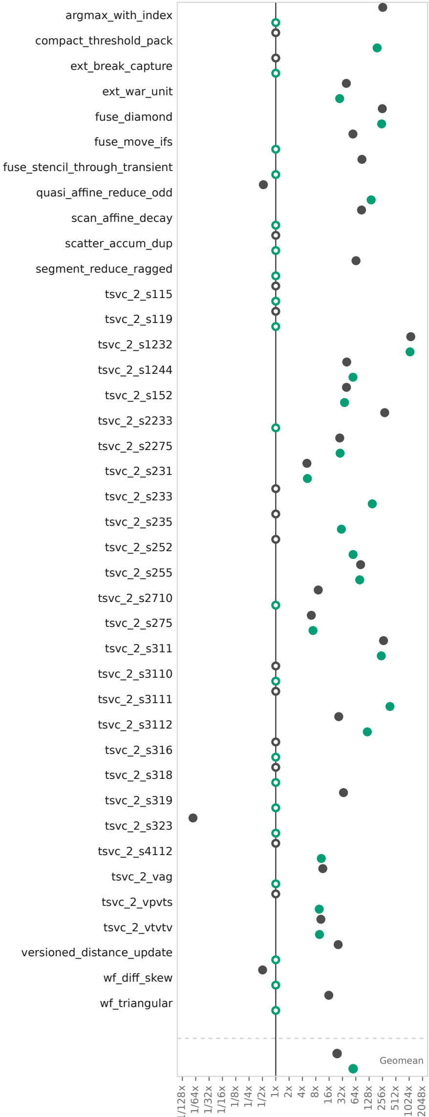
Qwen3.8-27B
