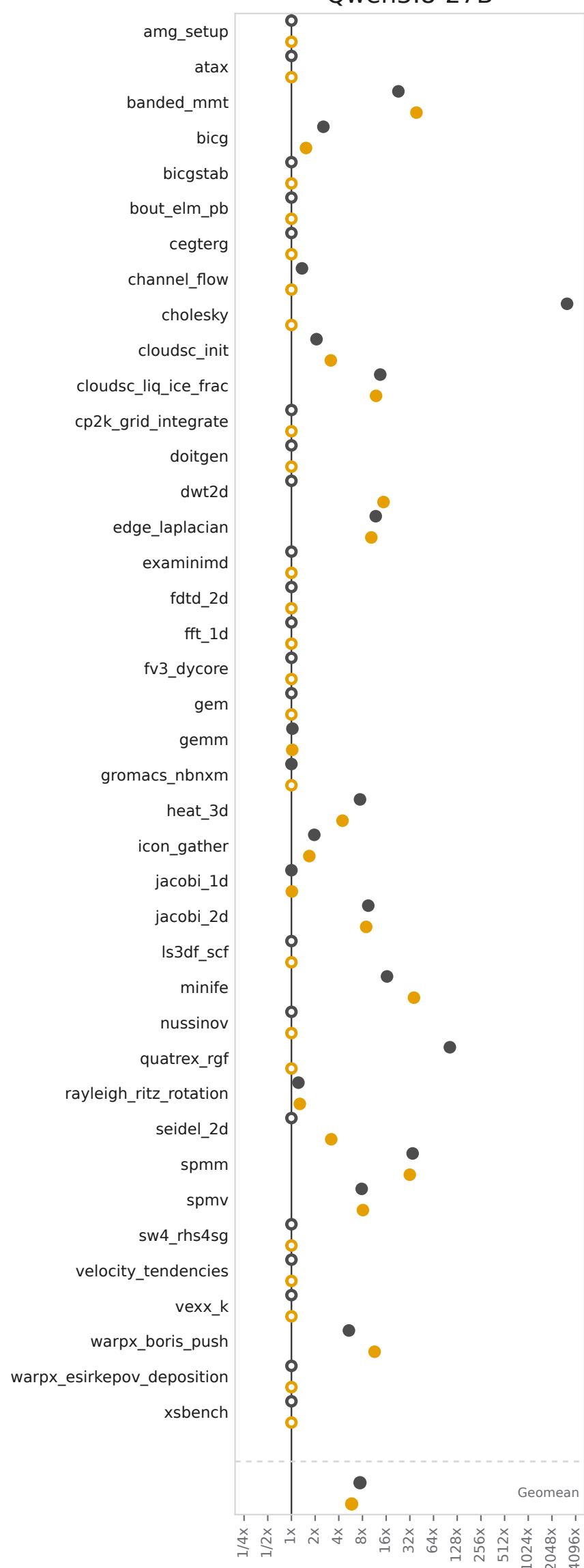
Qwen3.8-27B
