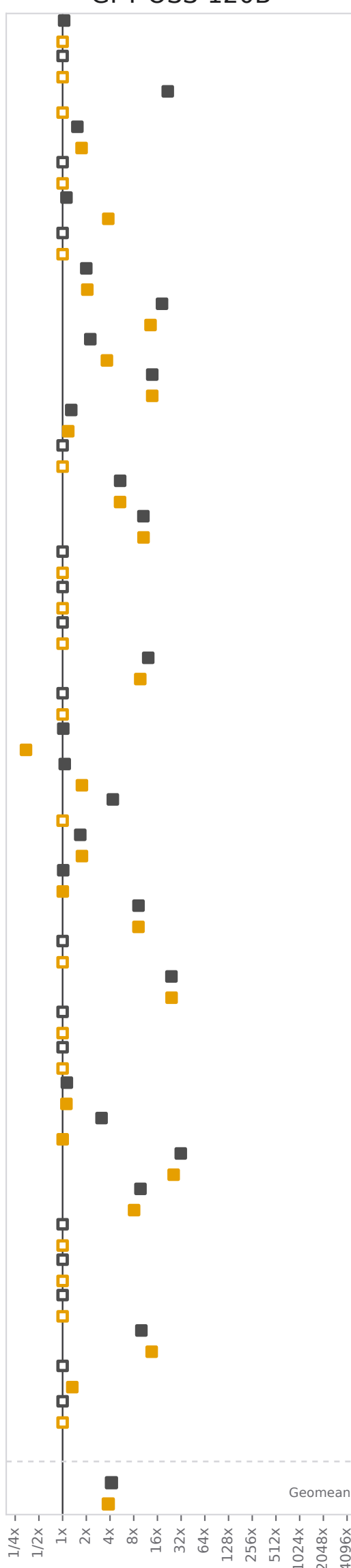
GPT-OSS-120B
