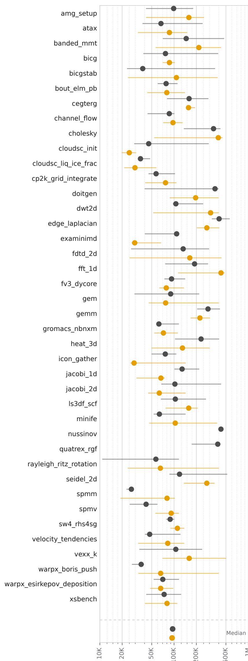
Tokens Spent
