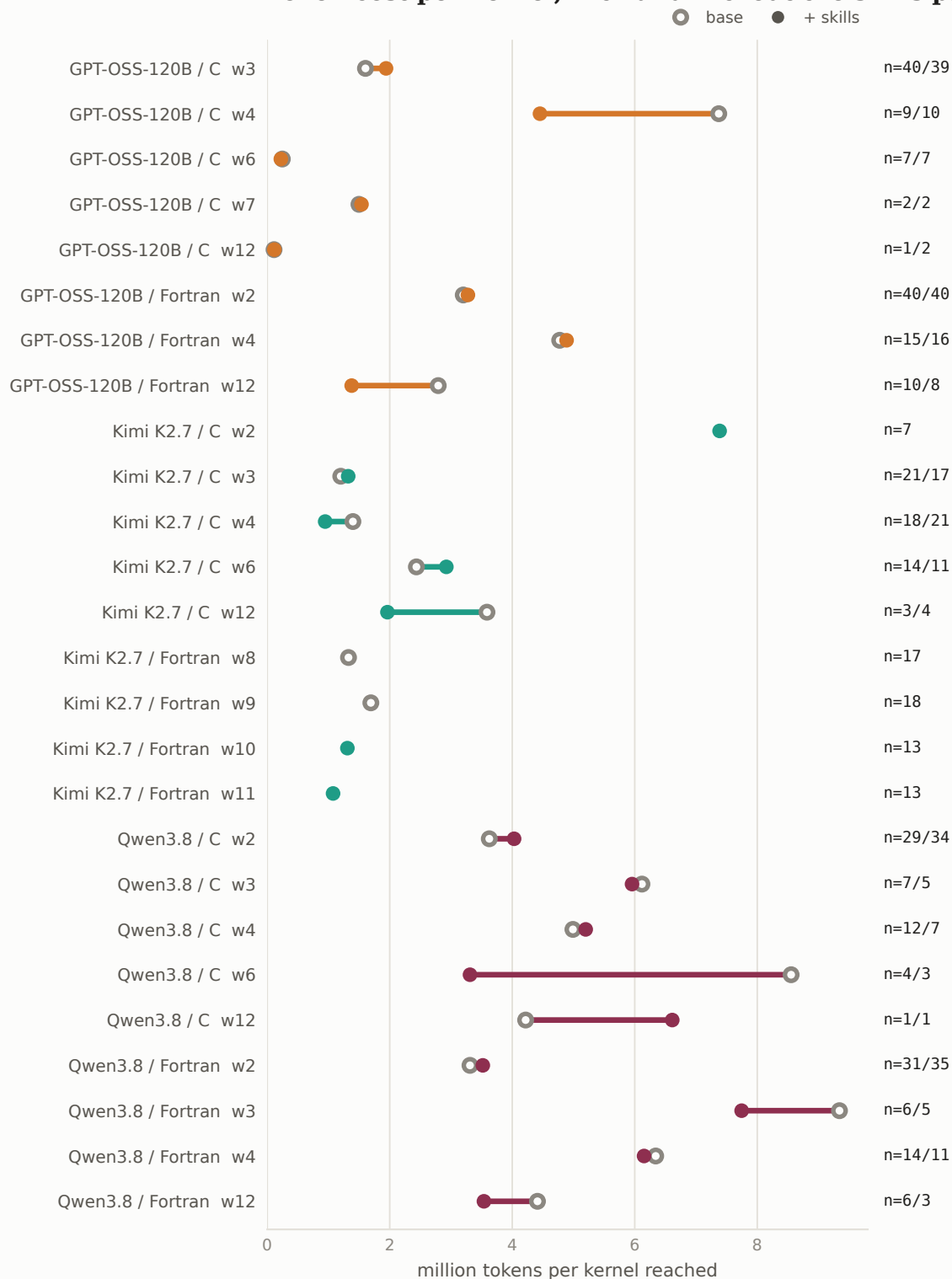
Token cost per kernel, with and without the skills packet
