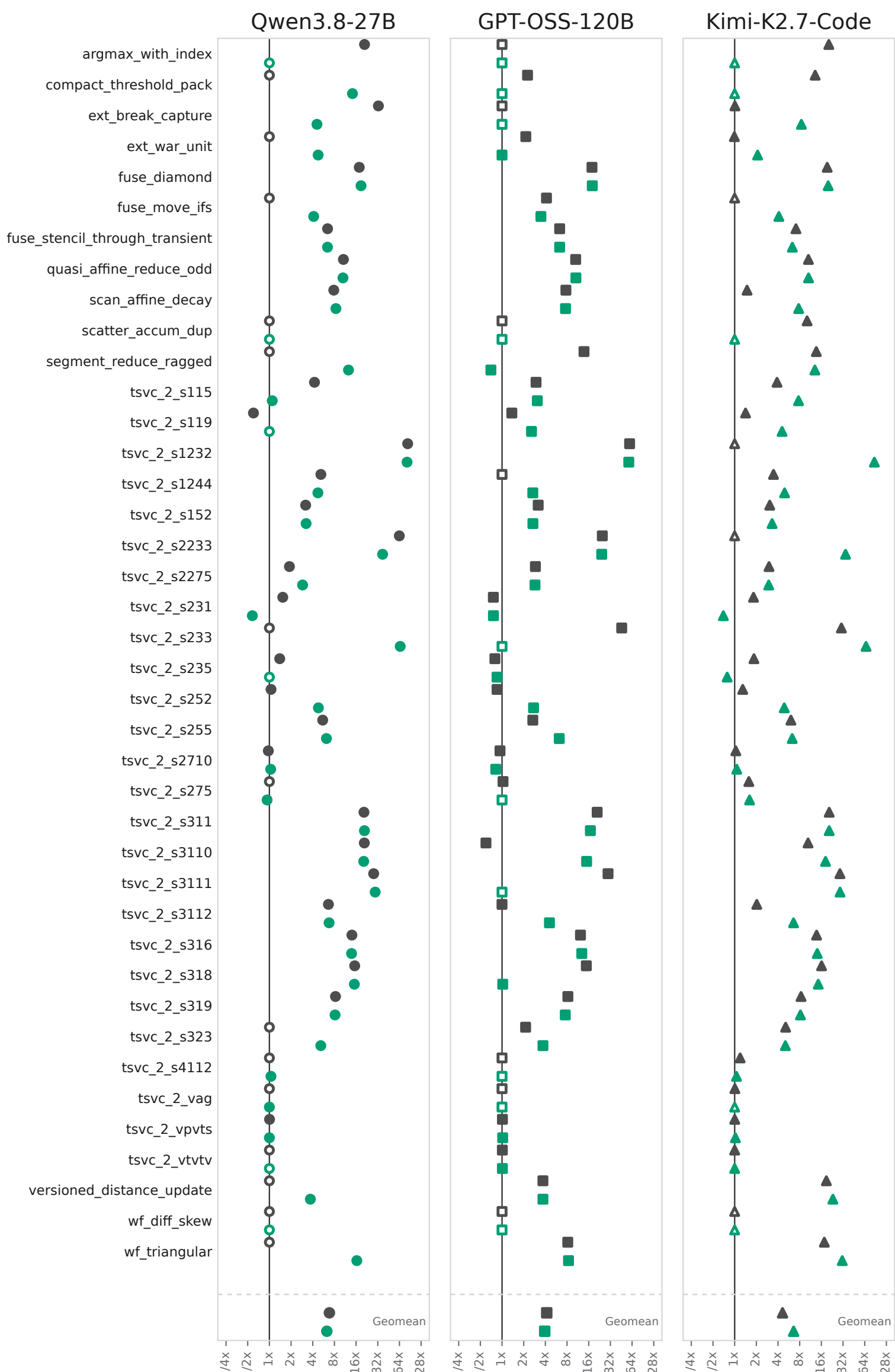
Speed-Up vs Numba
