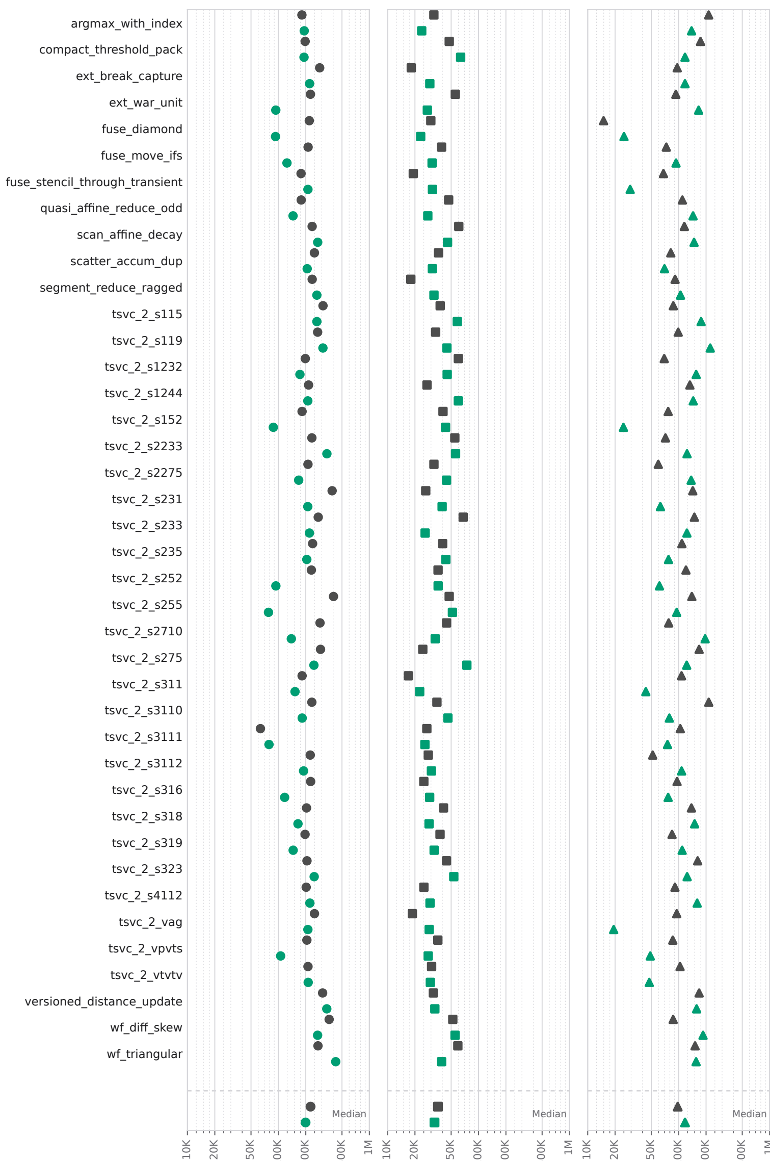
Tokens Spent
