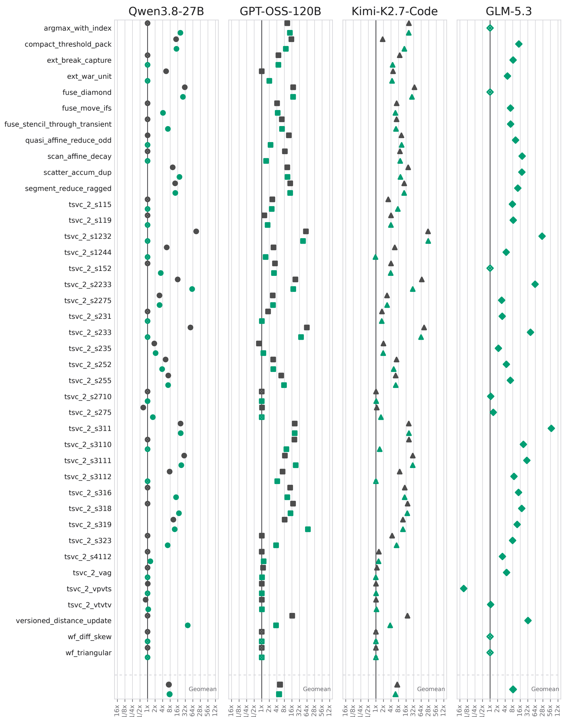
Speed-Up vs Numba
