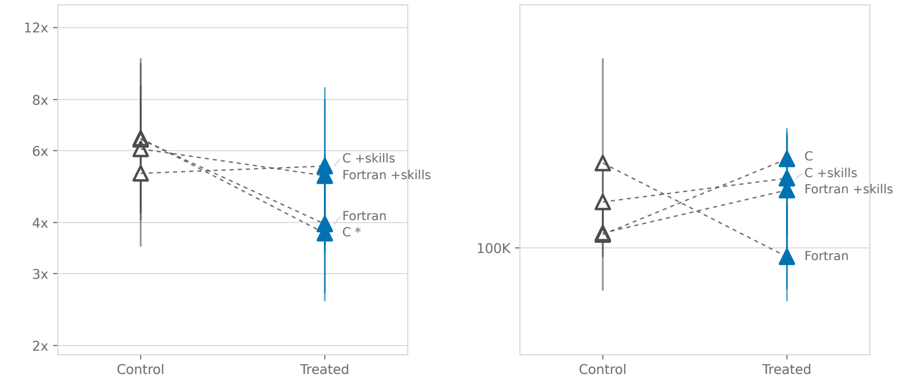
Kimi-K2.7-Code
