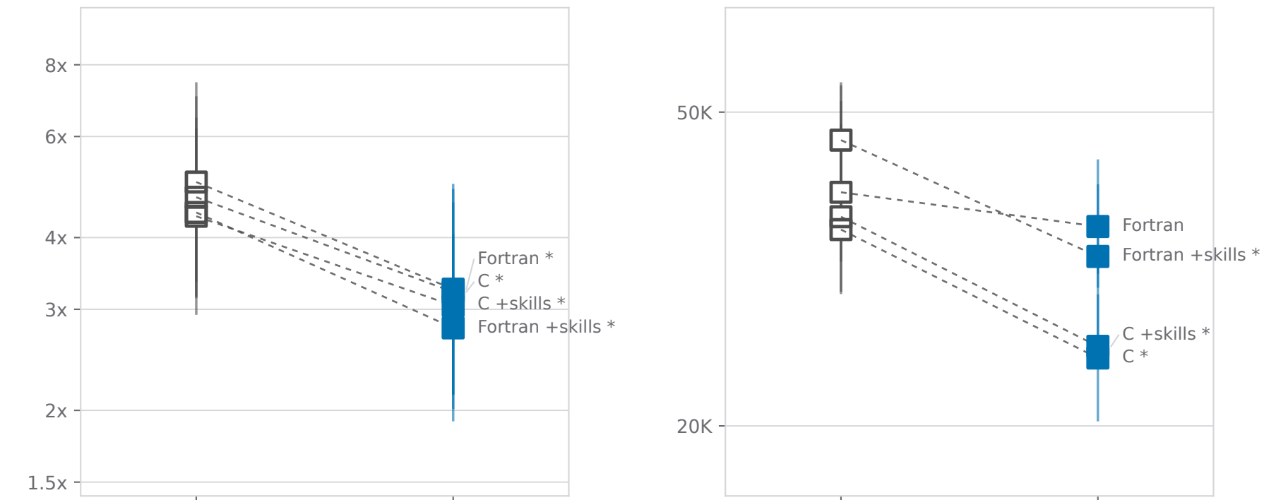
GPT-OSS-120B
