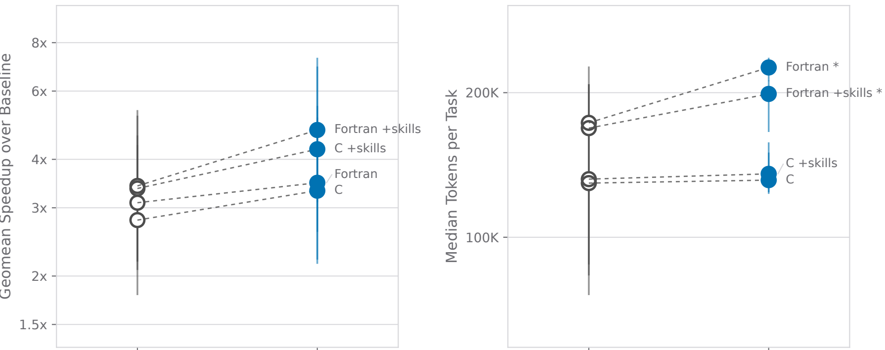
Qwen3.8-27B
