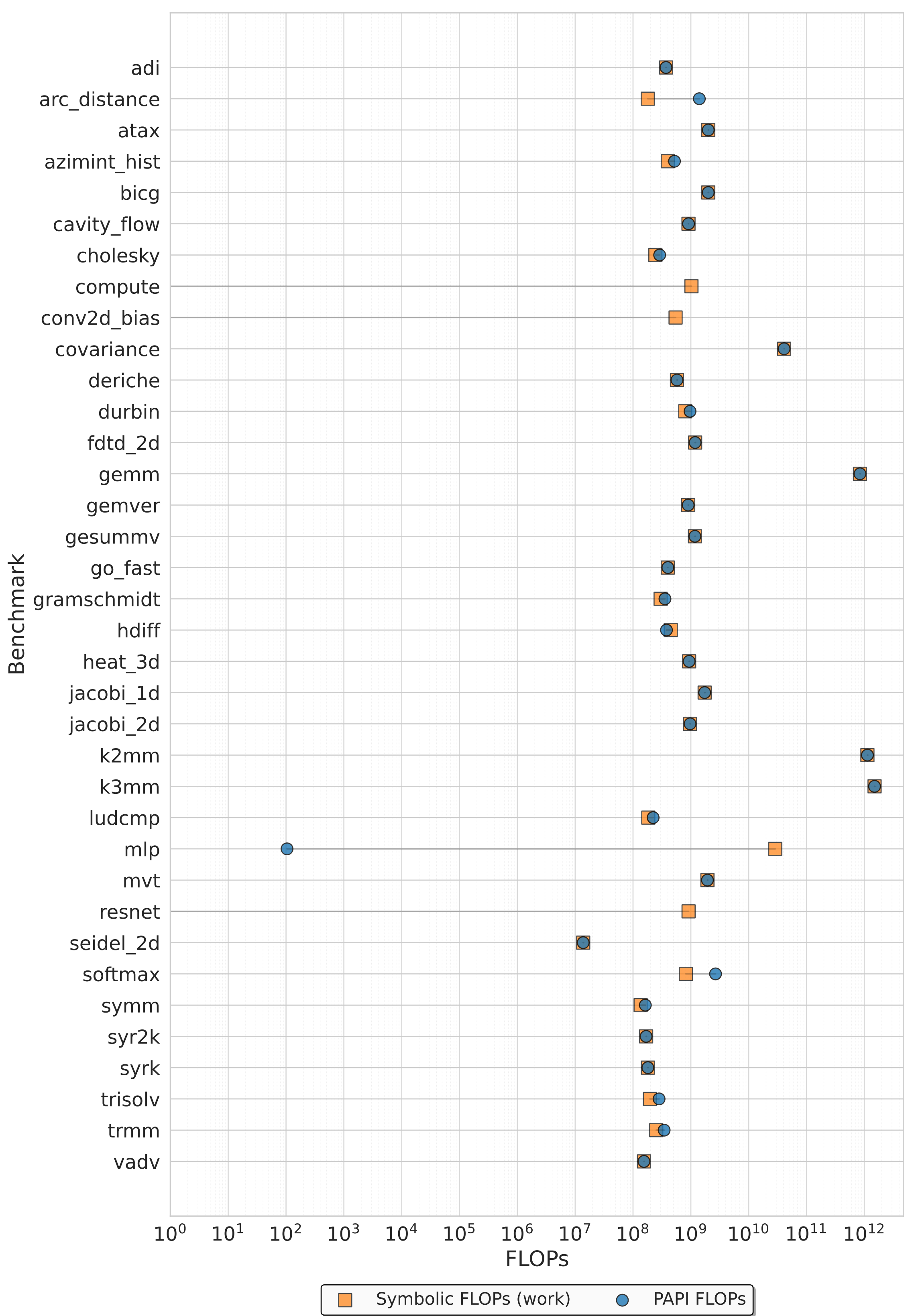
FLOPs Obtained Through Hardware Counters vs Symbolic Analysis
