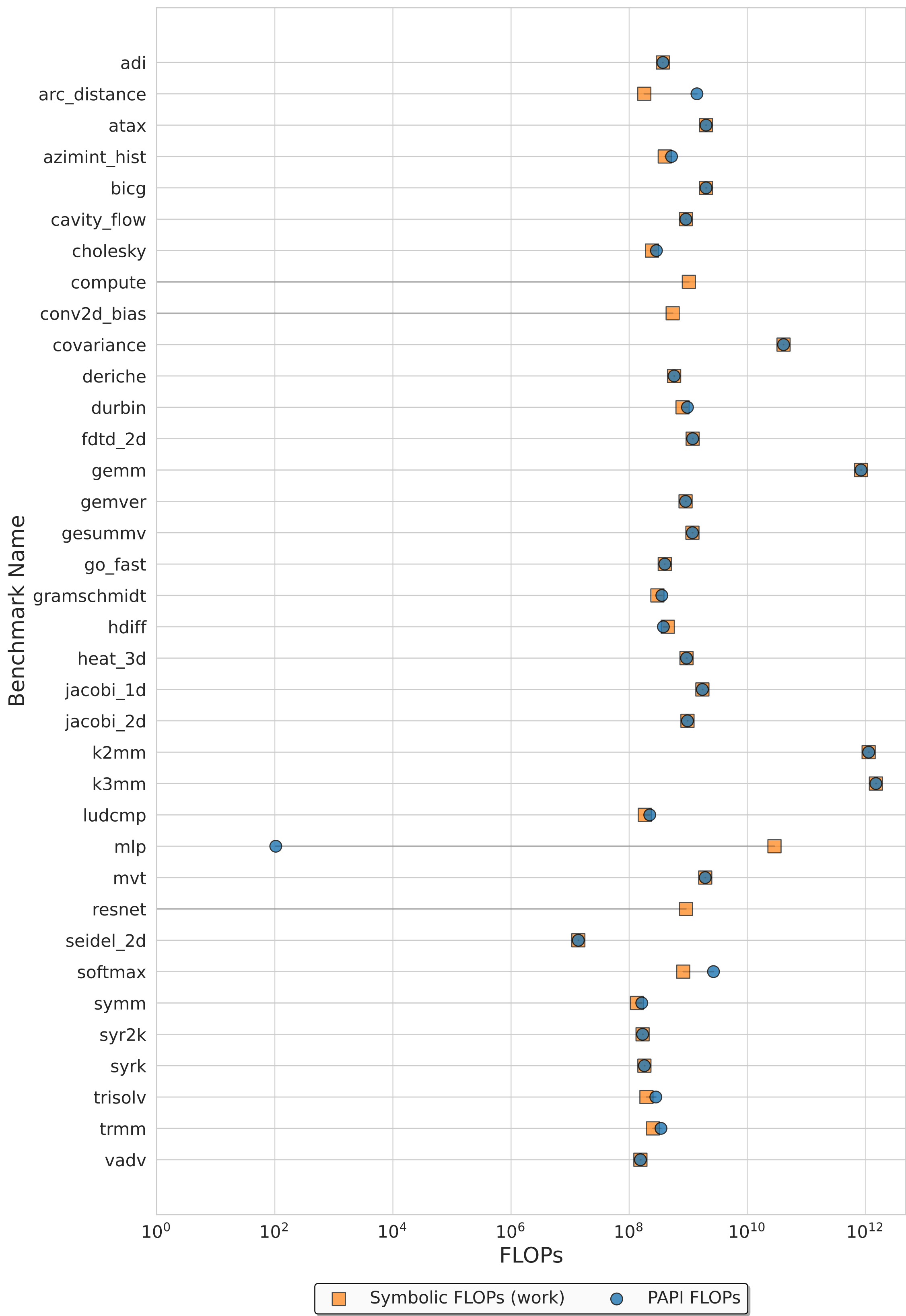
FLOPs Obtained Through Hardware Counters vs Symbolic Analysis
