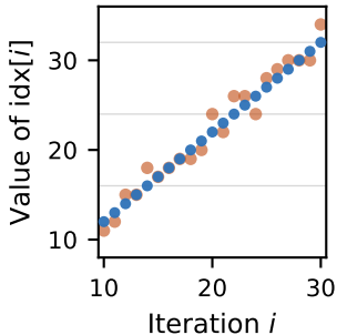
Access Sequence
