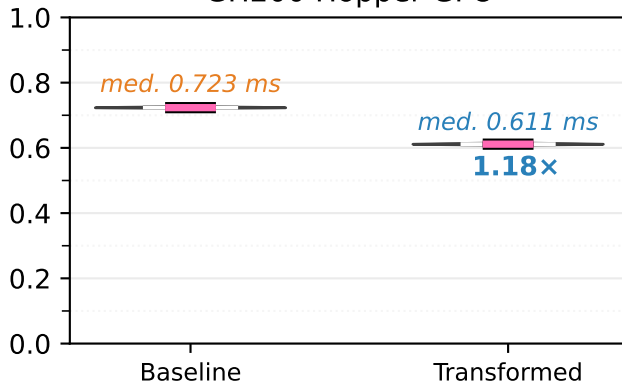
GH200 Hopper GPU
