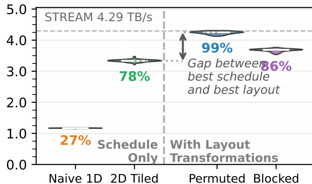
MI300A GPU
