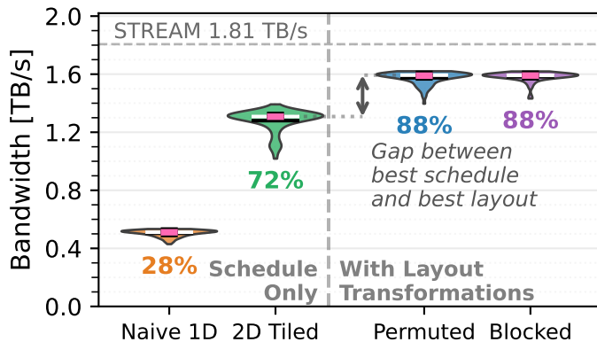
GH200 Grace CPU
