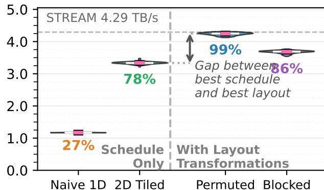
MI300A GPU
