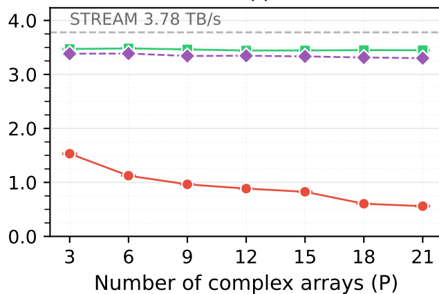
GH200 Hopper GPU
