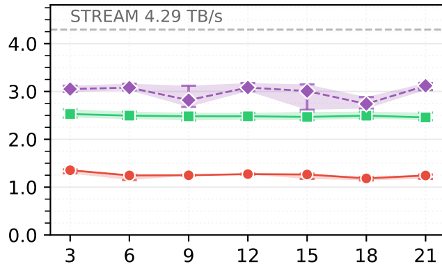
MI300A GPU
