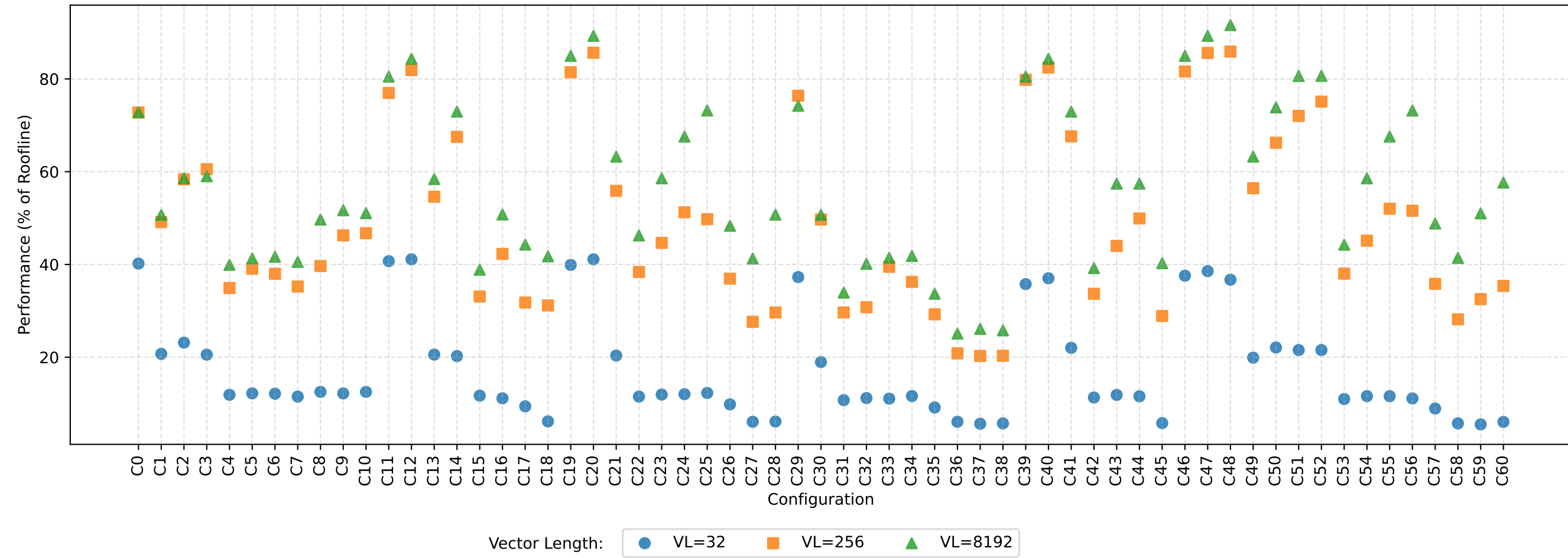
Roofline Efficiency per Vector Unit and L1 Configuration
