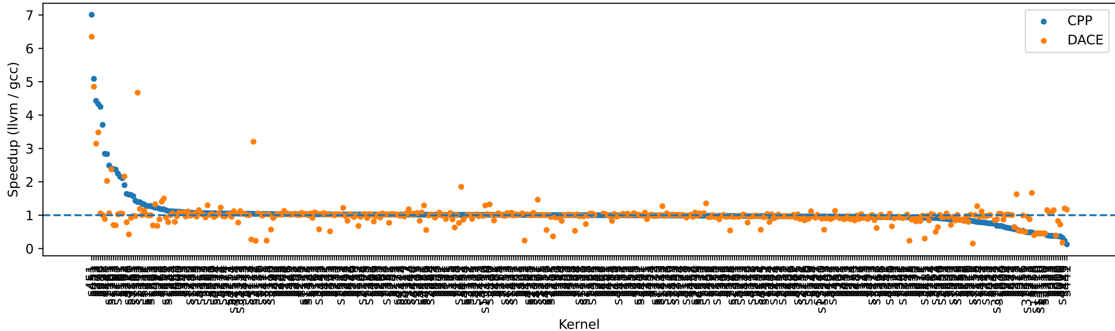
GCC speedup over LLVM: CPP vs DACE (aligned by kernel)
