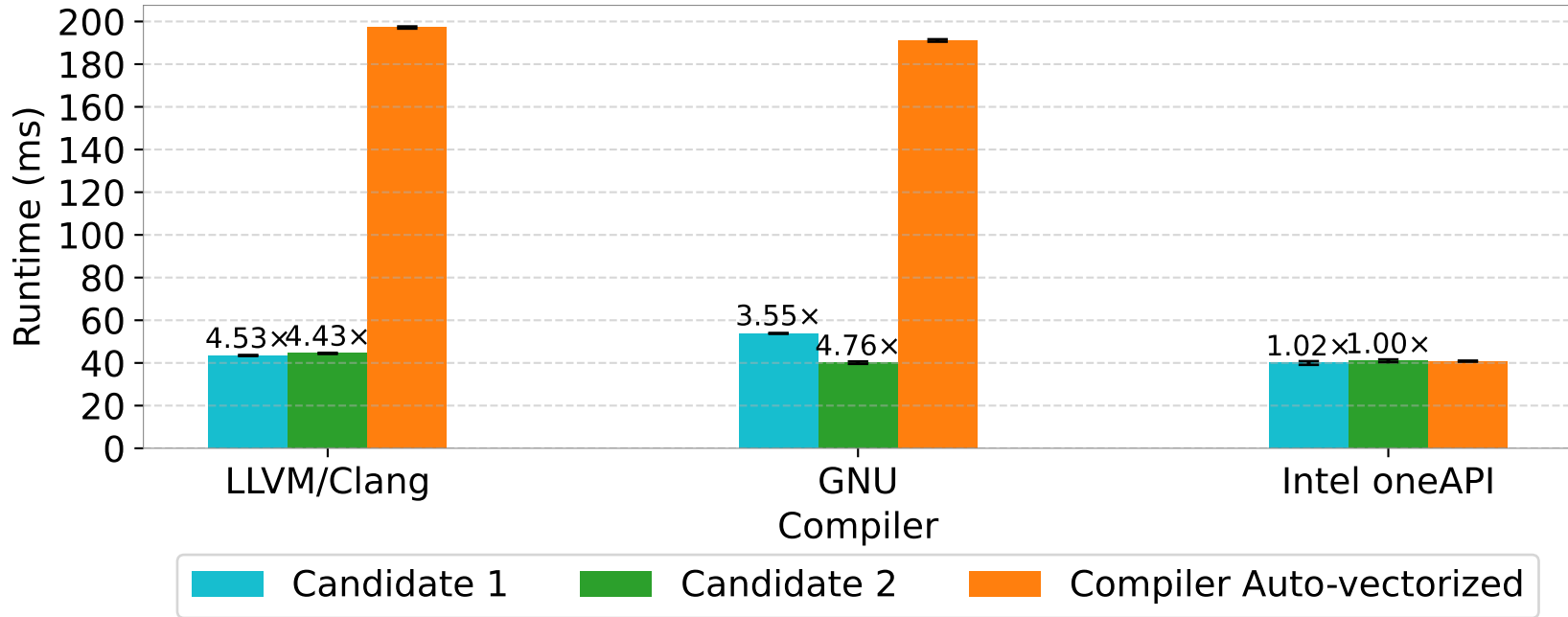
TSVC-2 Benchmark s441 Runtime Comparison
