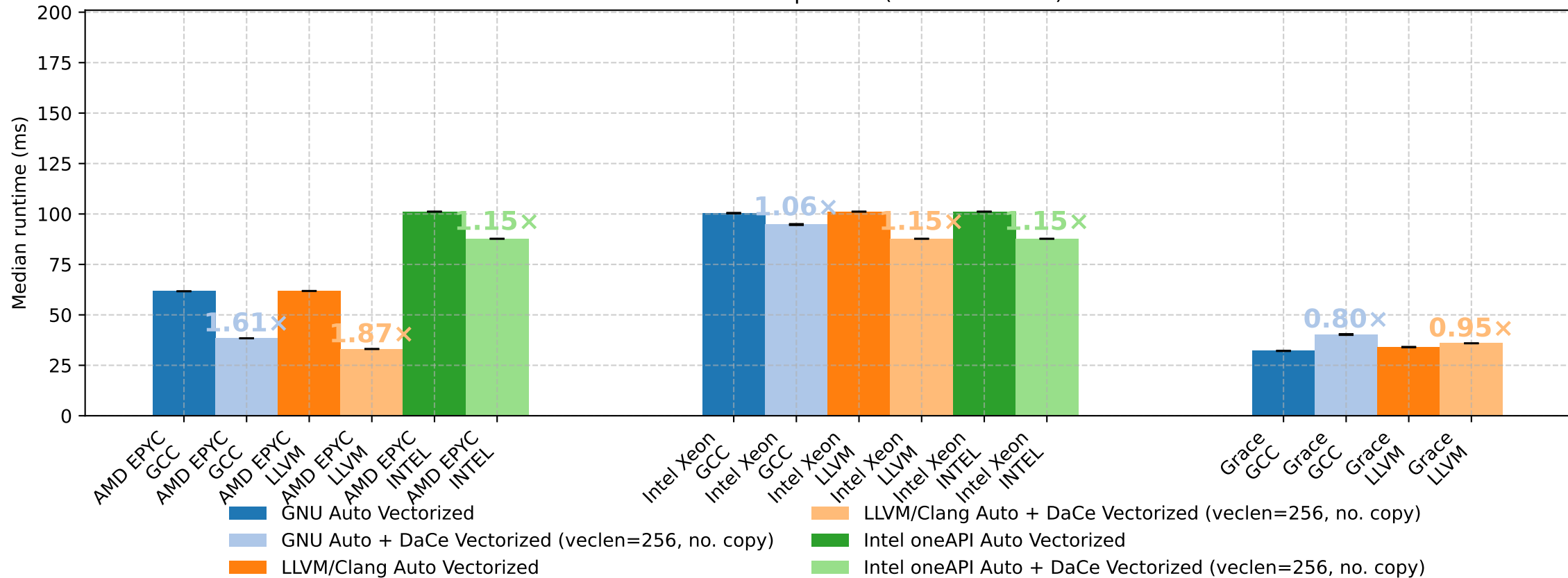
Vectorization Comparison (Size=9437184)
