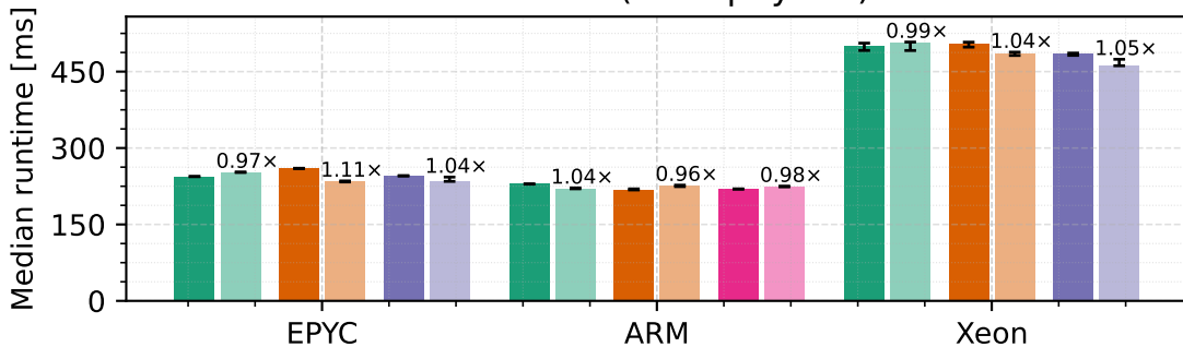
Rain Evaporation
