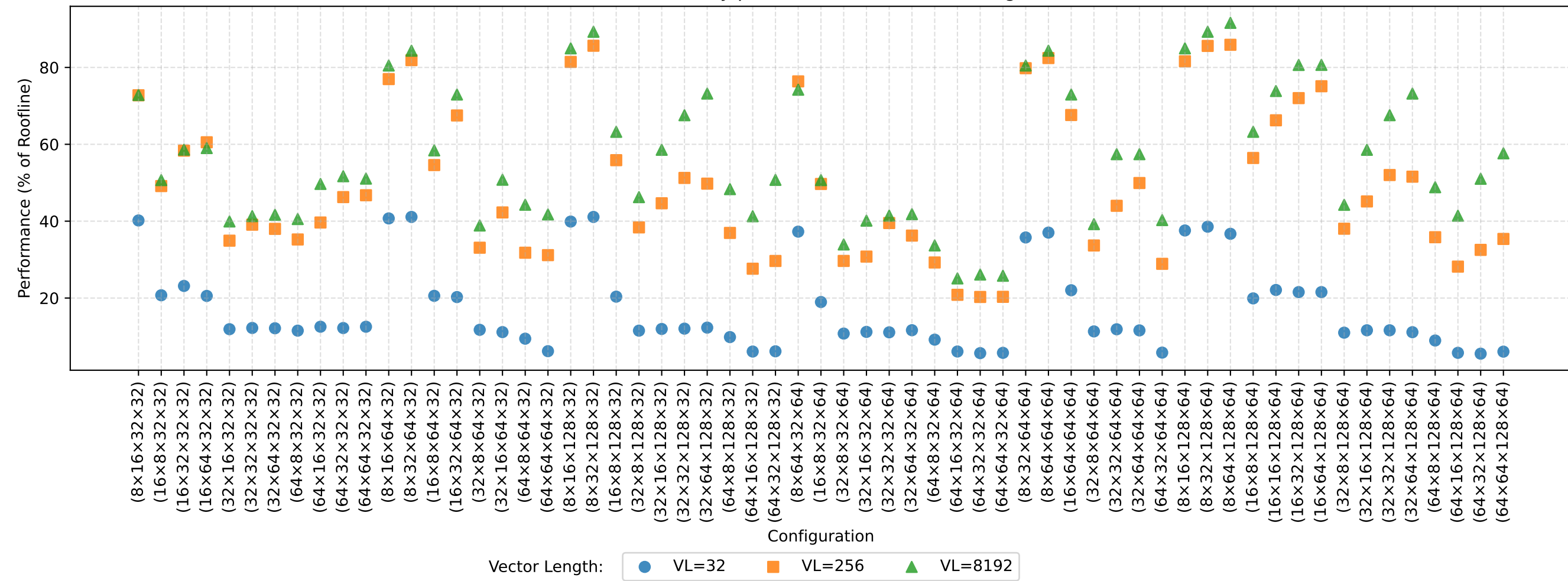
Roofline Efficiency per Vector Unit and L1 Configuration
