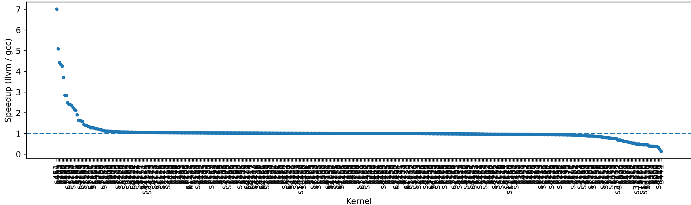
GCC speedup over LLVM (CPP variants)
