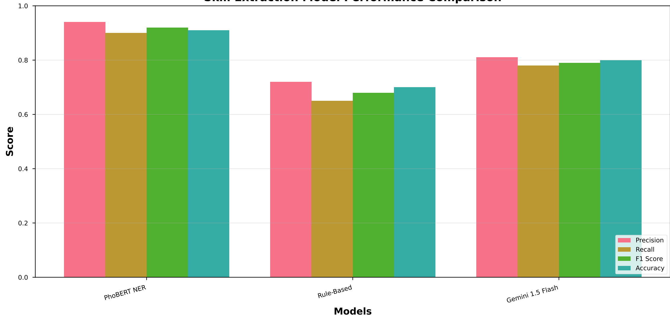
Skill Extraction Model Performance Comparison
