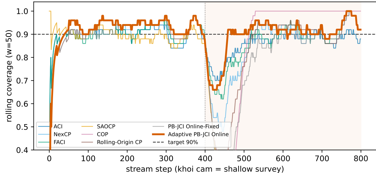
Astro: baseline hien dai vs Adaptive PB-JCI Online (deep->shallow shift)
