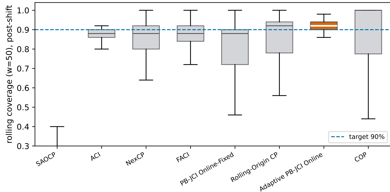
C. Boxplot: spread rolling-coverage/method (hep+giua 90% = it dao dong)
