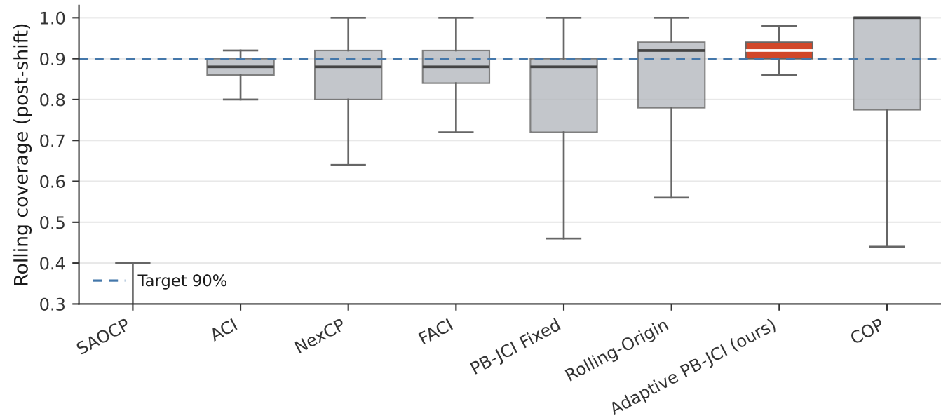
Coverage stability by method (tight box near 90% = stable)
