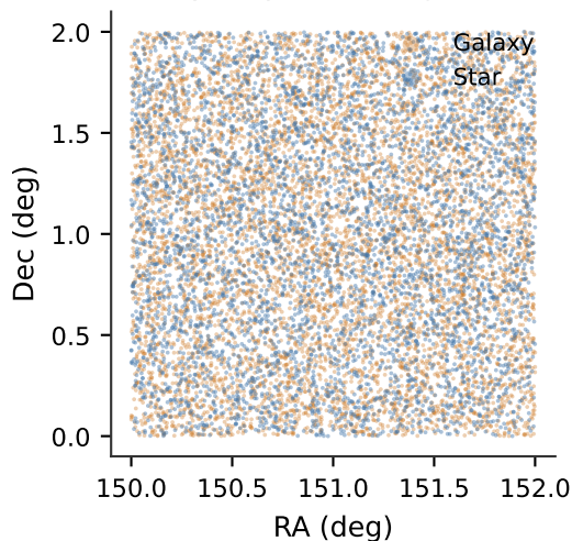
(c) Completeness model = induced depth shift
