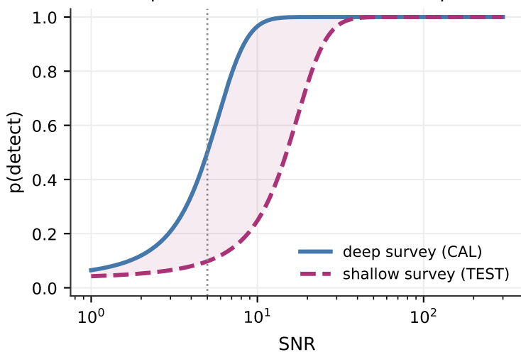
(c) Completeness model = induced depth shift
