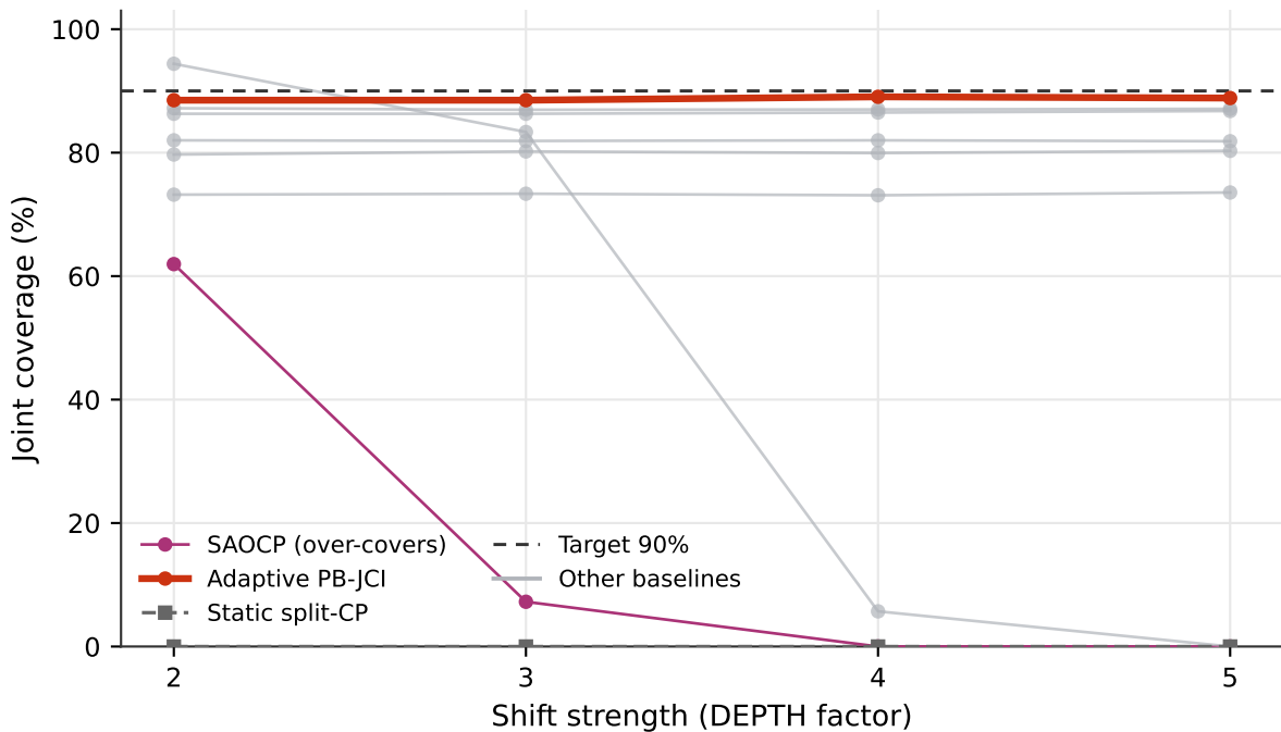
Coverage vs shift strength
