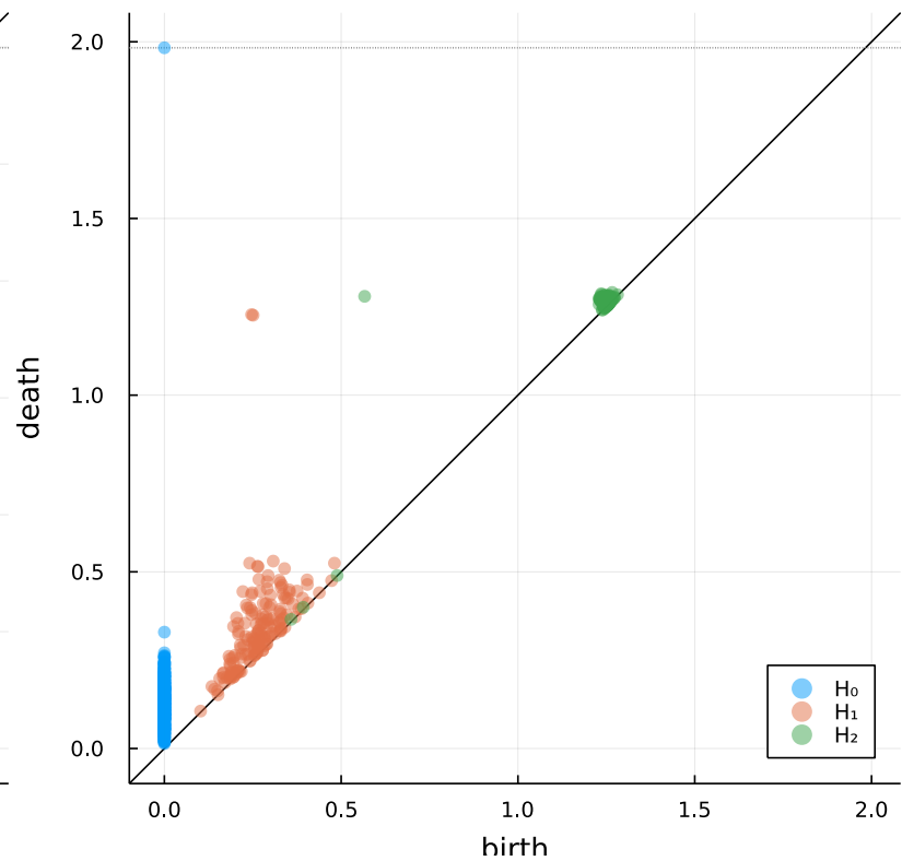
Torus Distance
