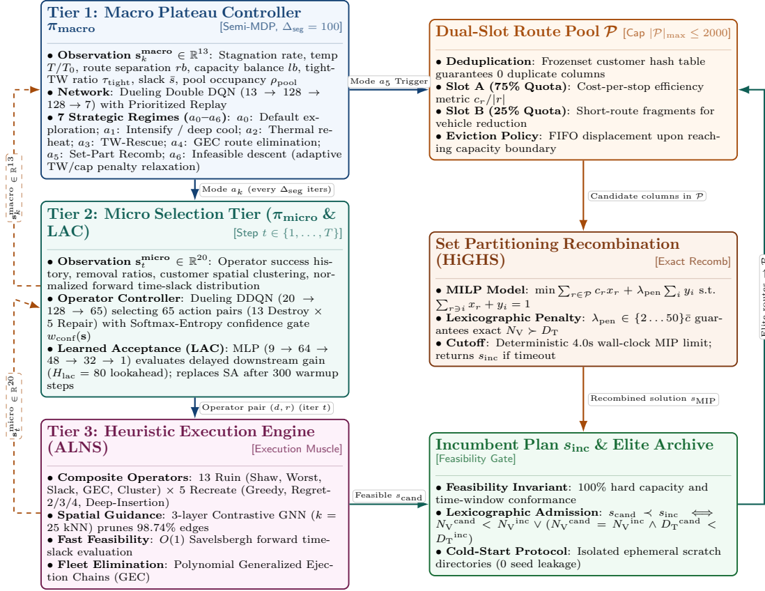
FIGURE 1. Tri-Level Hybrid DDQN-ALNS control architecture. Solid downward arrows represent hierarchical control and data dispatch across tiers. Dashed upward arrows represent state feedback signals consumed by the Macro and Micro RL training loops. The Macro tier operates over segment options \Delta_{\text{seg}} = 100 ; the Micro and Heuristic tiers execute per iteration t .
