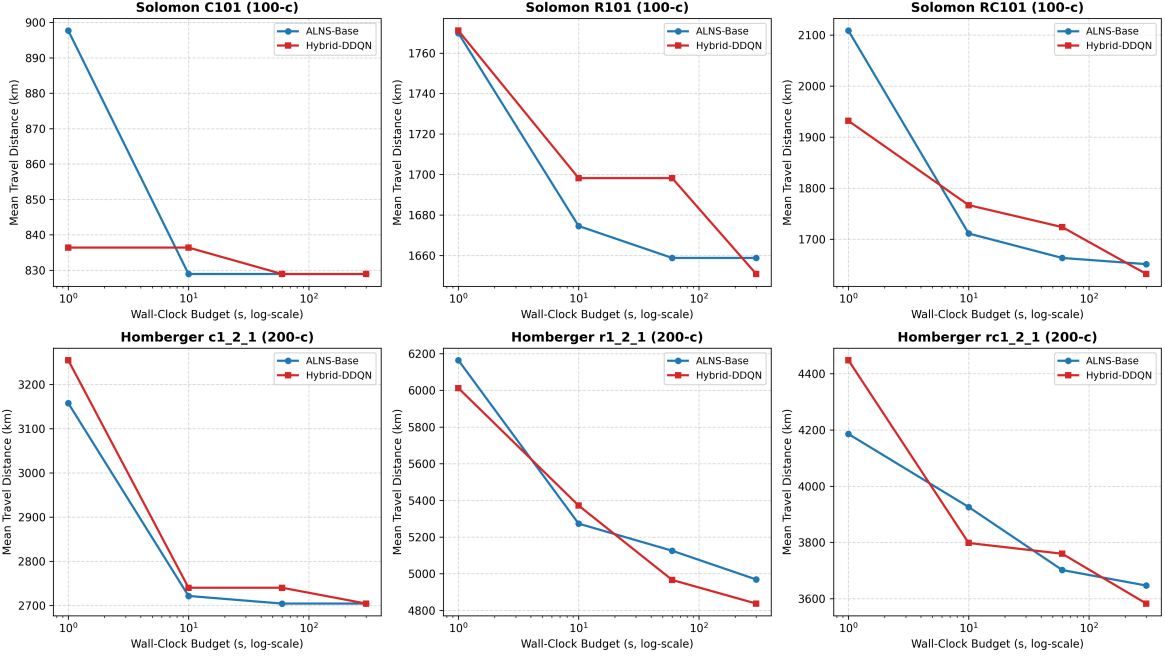
Equal wall-clock anytime convergence curves: Mean travel distance ( TD ) over wall-clock time t \in [1, 300] s across representative 100- and 200-customer topologies (C101, R101, RC101, c1_2_1, r1_2_1, rc1_2_1, N = 5 seeds, log-scale).
