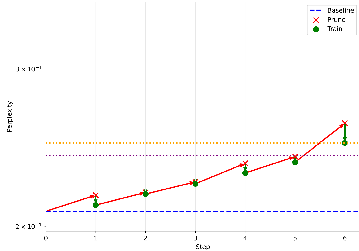
Iterative_Pruning Pruning Progression
